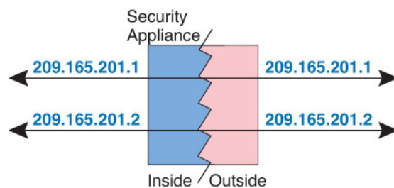
Figure 27: Identity NAT
