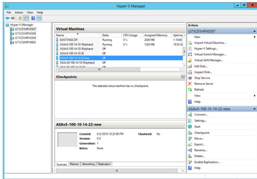
Figure 4: Hyper-V Manager
