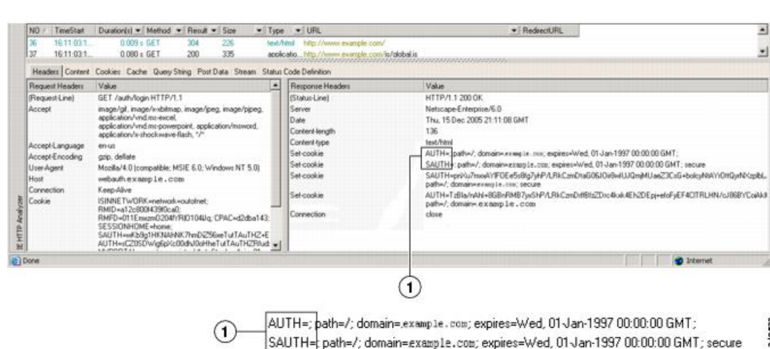
Figure 3: Authorization Cookies in Sample HTTP Analyzer Output
