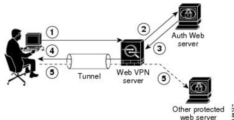
Figure 10: SSO Authentication Using HTTP Forms
