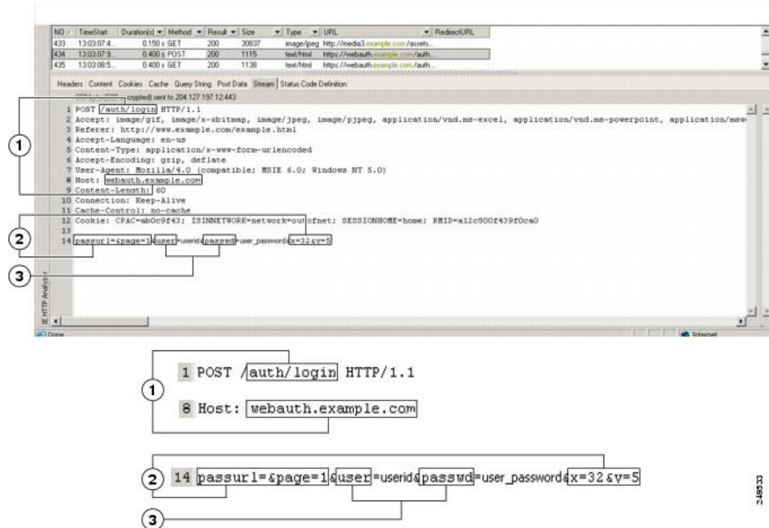
Figure 11: Action-uri, hidden, username and password parameters
