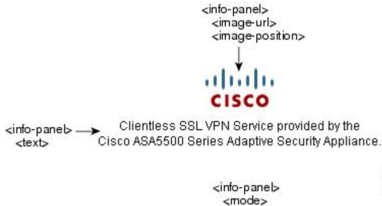
Figure 16: Information Panel on Logon Screen and Associated XML Tags
