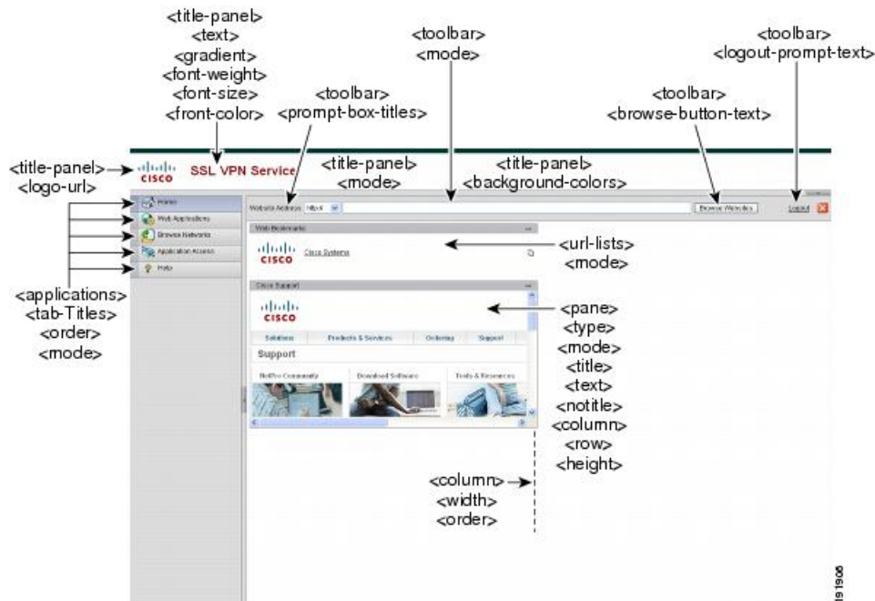
Figure 17: Portal Page and Associated XML Tags
