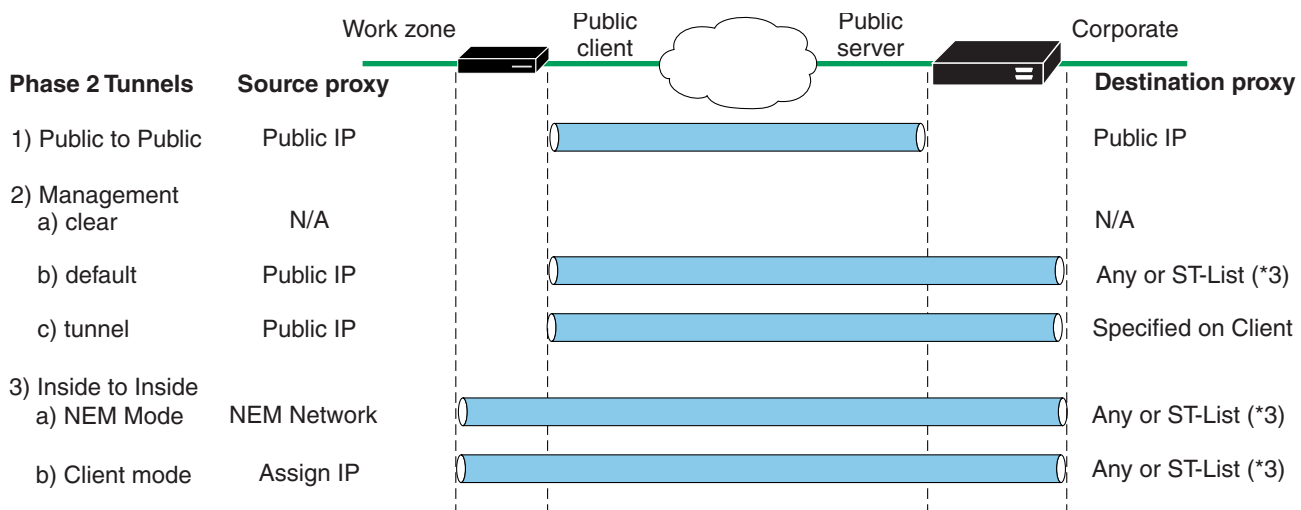
Figure 1-1 Easy VPN Hardware Client Tunneling Options for the Cisco ASA 5505
