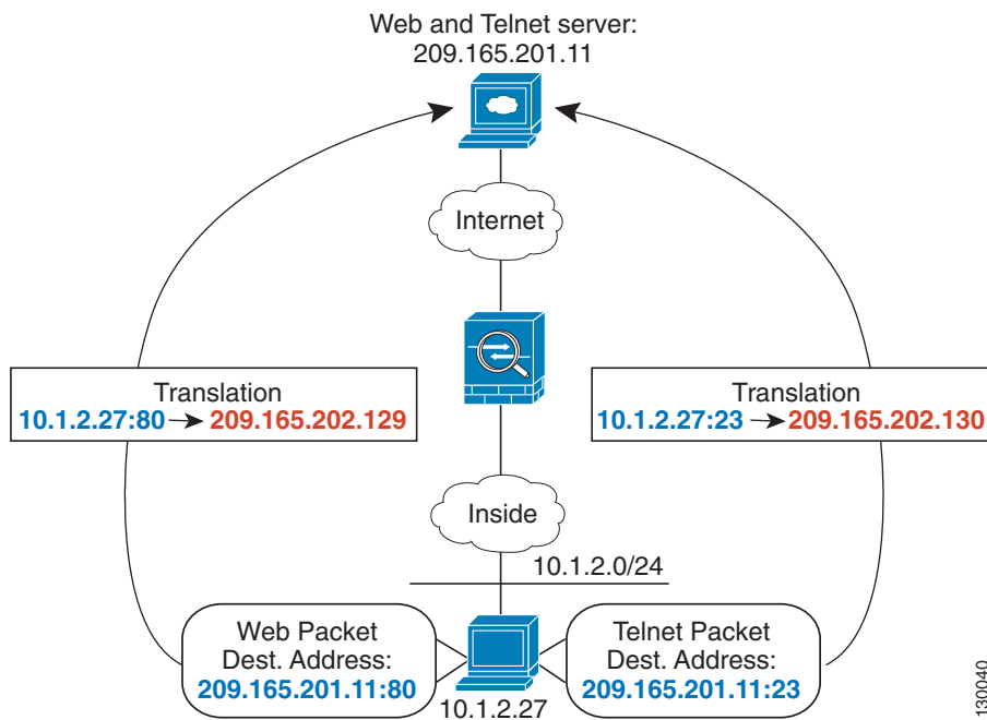
Figure 1-2 Twice NAT with Different Destination Ports
