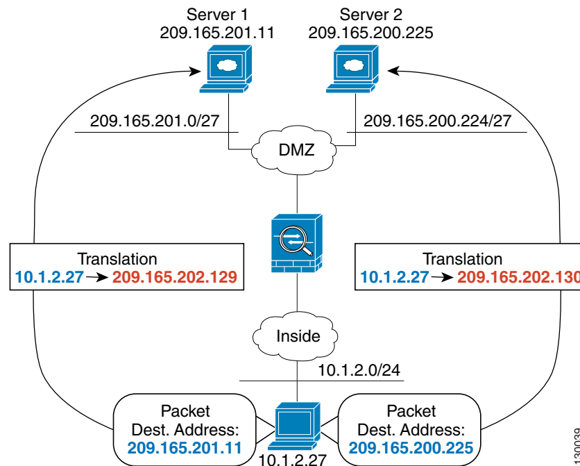
Figure 1-1 Twice NAT with Different Destination Addresses
