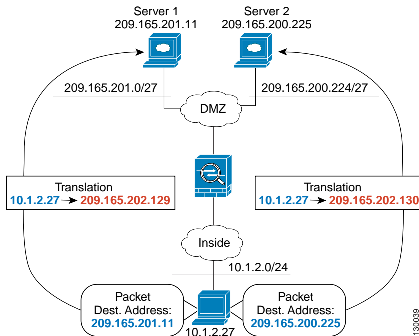
Figure 1-1 Twice NAT with Different Destination Addresses
