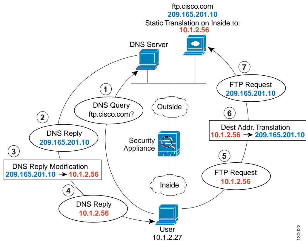
Figure 1-6 DNS Reply Modification Using Outside NAT
