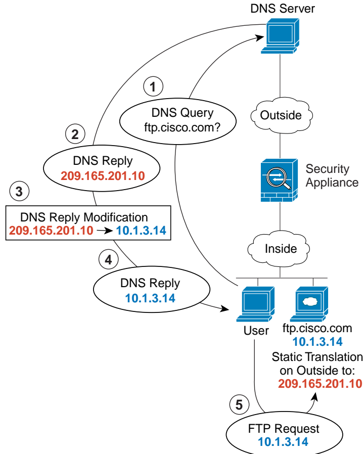
Figure 1-5 DNS Reply Modification
