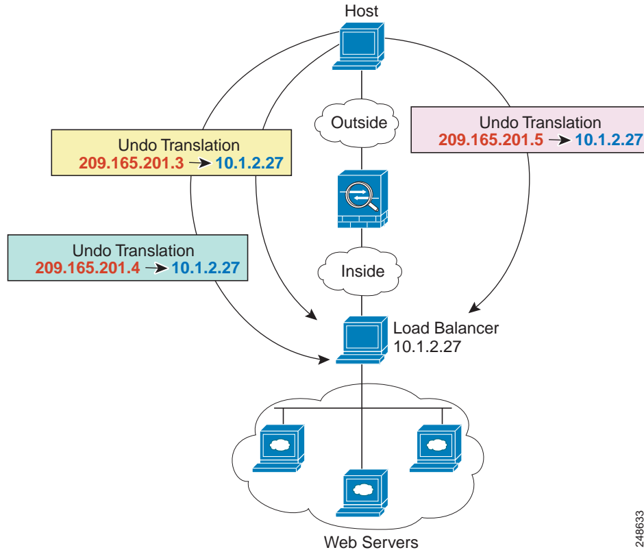
Figure 1-3 Static NAT with One-to-Many for an Inside Load Balancer
