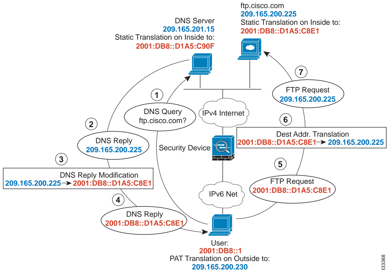
Figure 1-7 DNS Reply Modification Using Outside NAT
