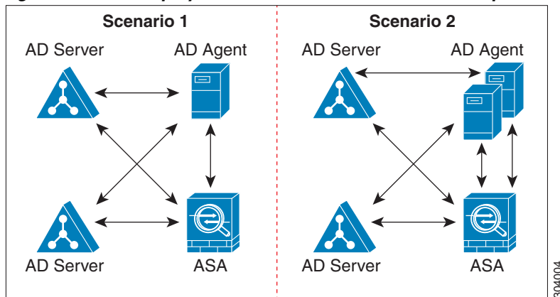
Figure 1-3 Deployment Scenario with Redundant Components
