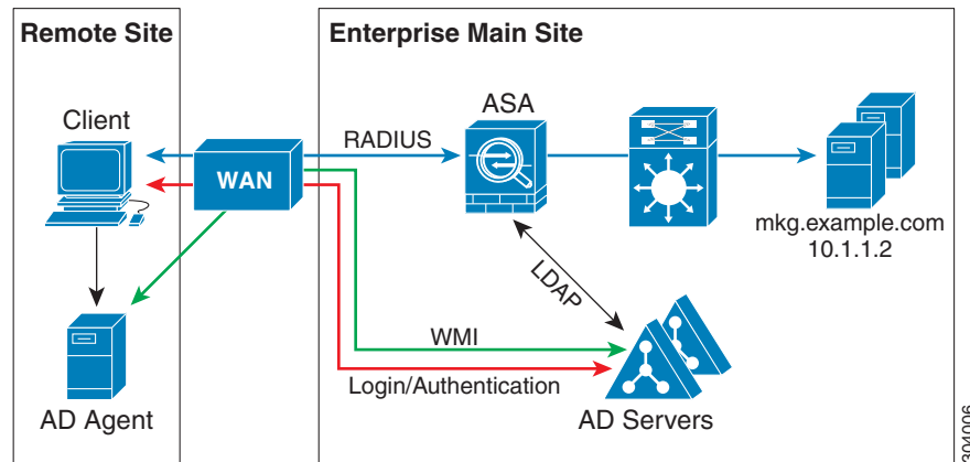
Figure 1-7 WAN-based Deployment with Remote AD Agent and AD Servers
