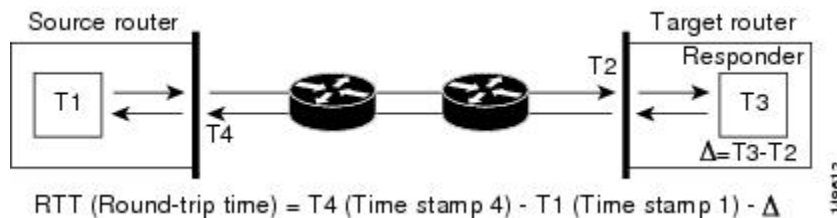
Figure 3: IP SLA Responder Time Stamping
