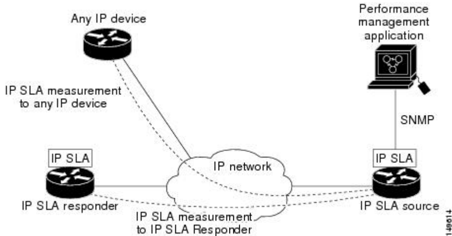
Figure 2: IP SLA Operations
