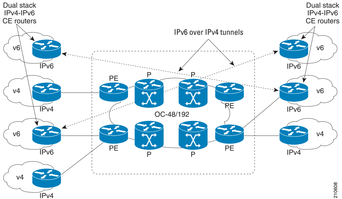
Figure 21 IPv6 Using Tunnels on the CE Routers
