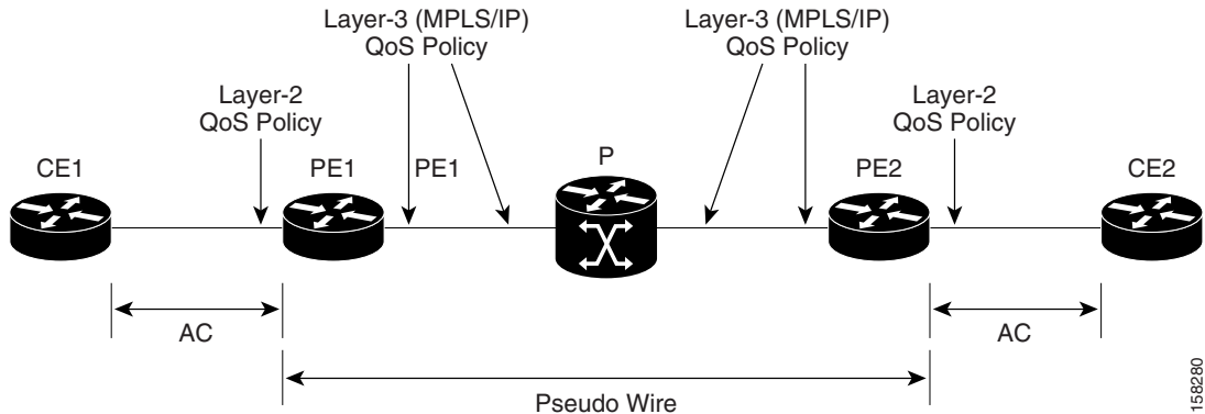
Figure 5 L2VPN QoS Feature Application
