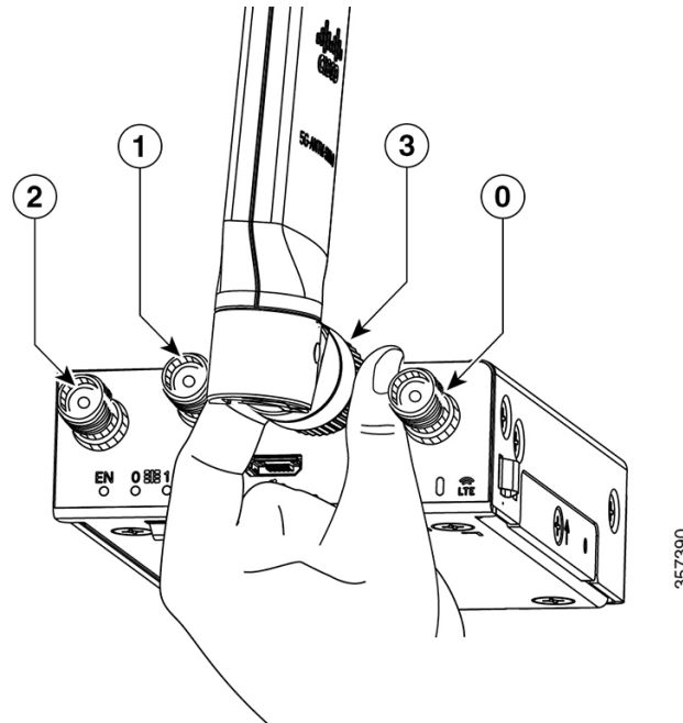
Figure 3: Attaching the antennas
