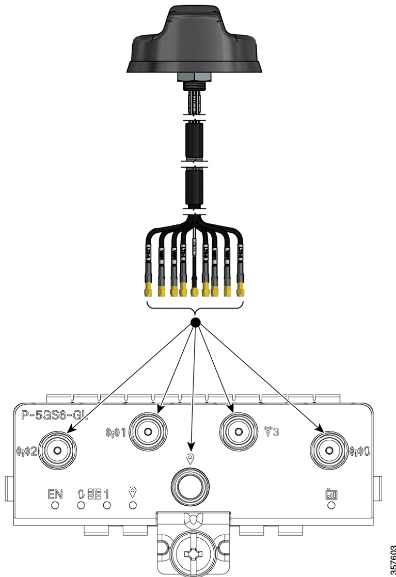
Figure 4: Attaching 5G NR Antenna (5G-ANTM-04-B) to P-5GS6-GL PIM
