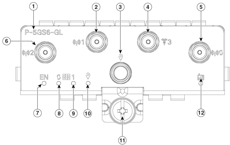
Figure 2: 5G Pluggable Interface Module - P-5GS6-GL
