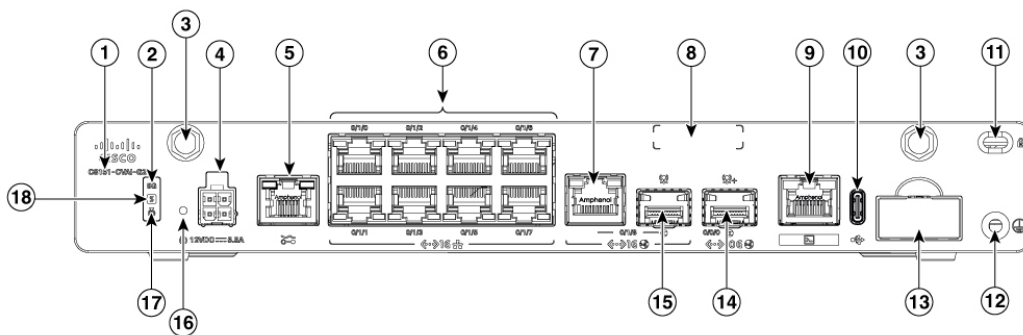
Figure 86: C8151-CVAI-G2 and C8151-CVAP-G2 - Front view
