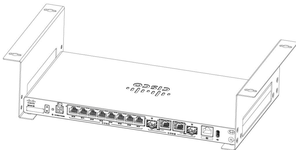
Figure 40: C8151-G2 and C8161-G2 with attached under desk mounting brackets
