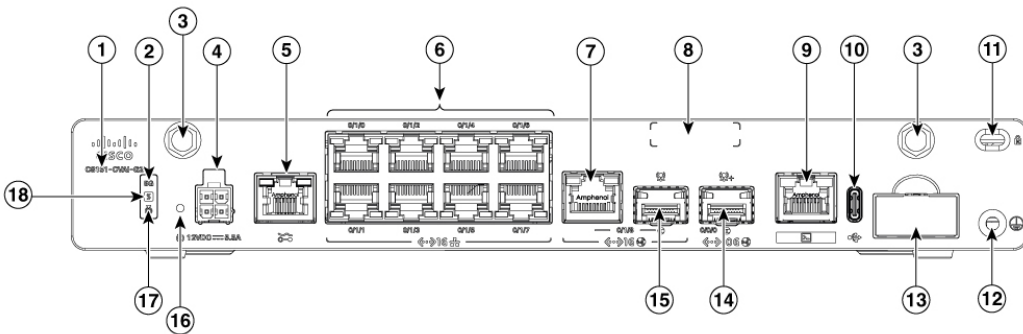
Figure 14: C8151-CVAI-G2 and C8151-CVAP-G2 - Front view
