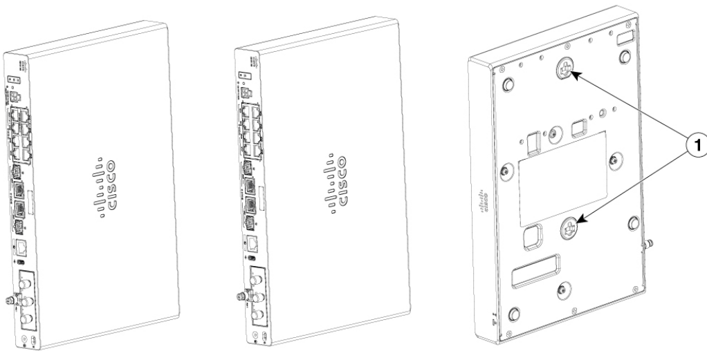
Figure 51: Wall mount using keyhole slots for C8151-G2 and C8161-G2
