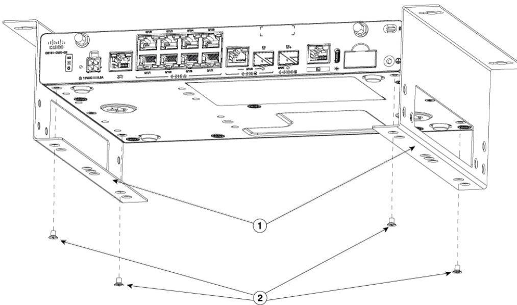
Figure 37: Under desk mounting brackets installation for C8151-CVAI-G2 and C8151-CVAP-G2
