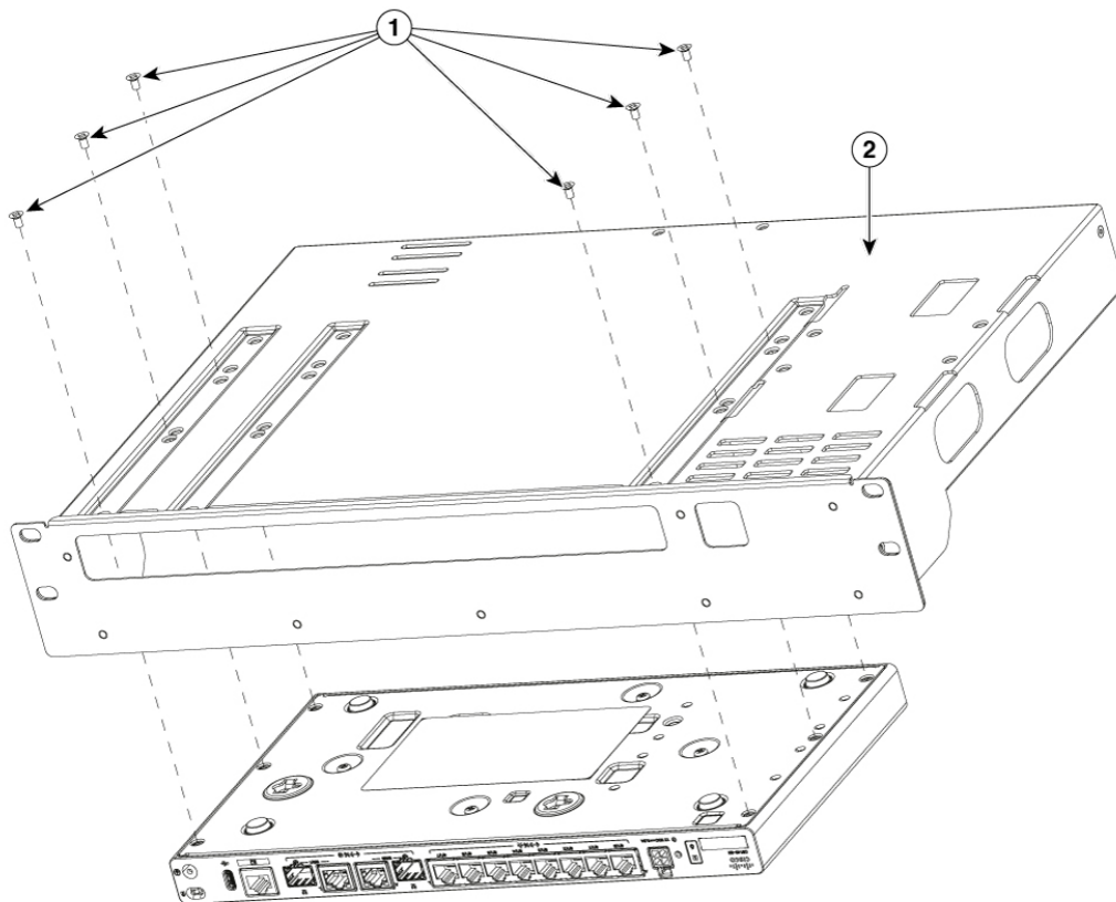
Figure 24: Rack mounting bracket installation for C8140-G2
