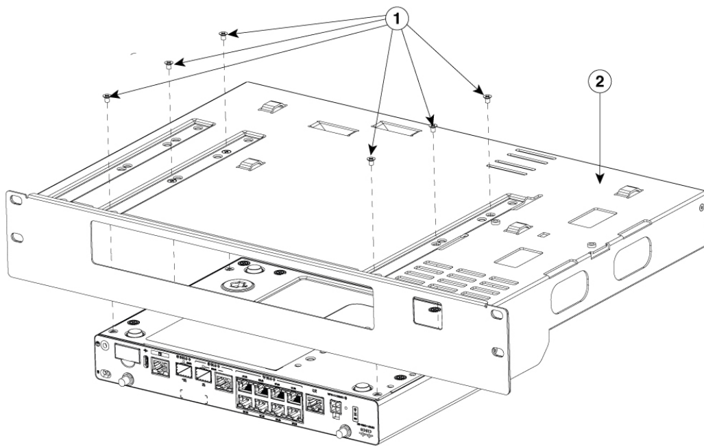
Figure 27: Rack mounting bracket installation for C8151-CVAI-G2 and C8151-CVAP-G2
