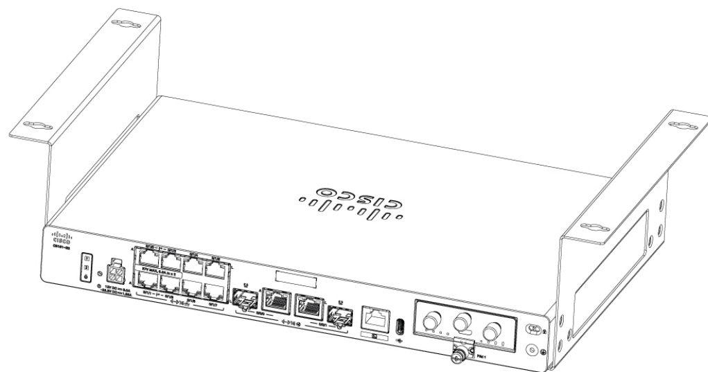
Figure 41: C8130-VAI-G2 and C8130-VAP-G2 with attached under desk mounting brackets
