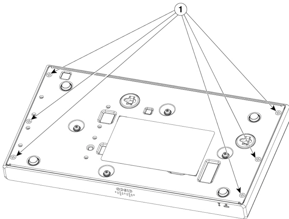
Figure 19: Removing screws from C8140-G2
