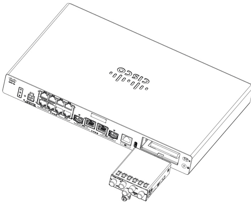
Figure 80: C8151-G2 and C8161-G2 with attached Pluggable Interface Module
