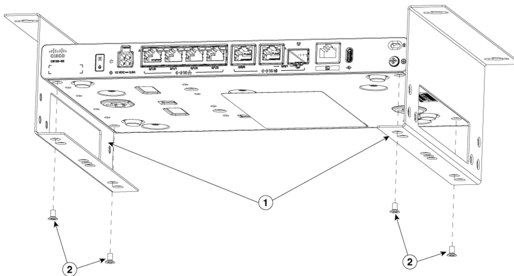
Figure 33: Under desk mounting brackets installation for C8130-G2 and C8131-G2
