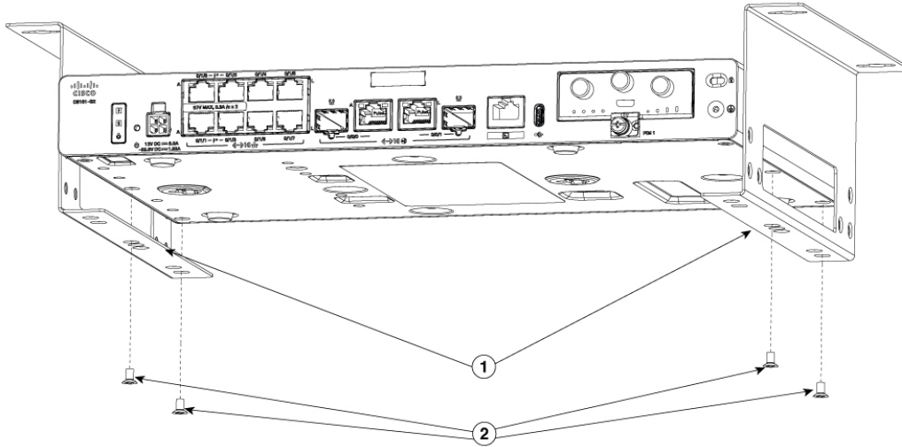
Figure 35: Under desk mounting brackets installation for C8151-G2 and C8161-G2
