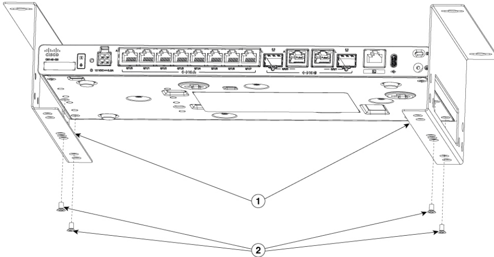
Figure 34: Under desk mounting brackets installation for C8140-G2
