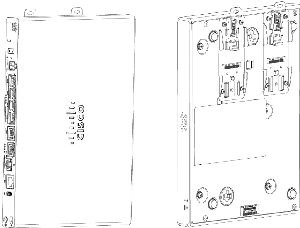
Figure 60: C8140-G2 with attached DIN rail brackets
