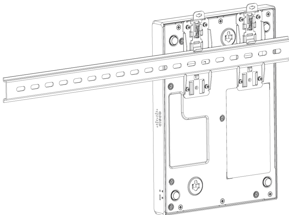
Figure 68: Mounting C8151-CVAI-G2 and C8151-CVAP-G2 using DIN rail brackets
