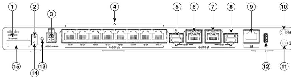
Figure 6: C8140-G2 - Front view
