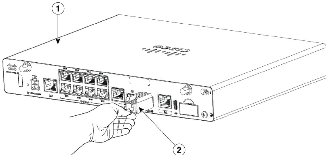
Figure 91: Hand Position for SFP-10G-ONT20-I Optical Removal
