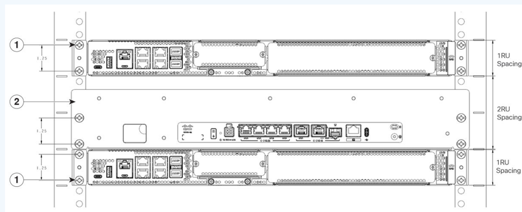
Figure 17: Rack-tray assembly
