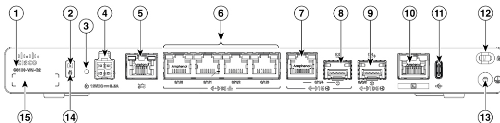
Figure 12: C8130-VAI-G2 and C8130-VAP-G2 - Front view
