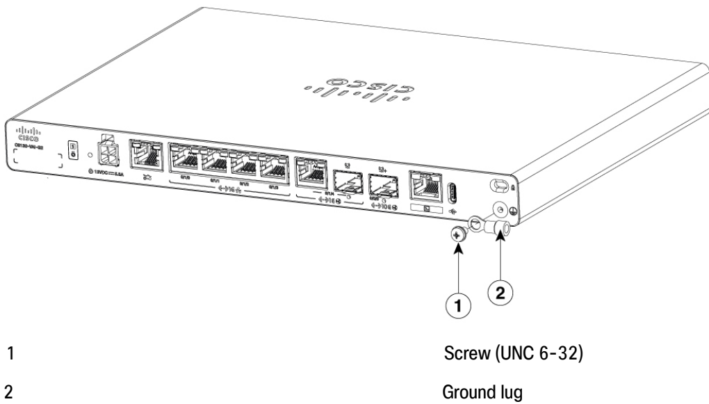
Figure 73: Chassis ground connection - C8151-CVAI-G2 and C8151-CVAP-G2
