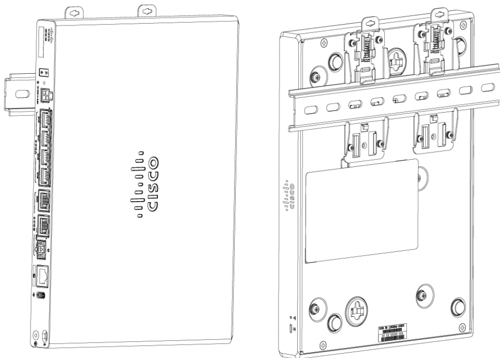
Figure 65: Mounting C8140-G2 using DIN rail brackets
