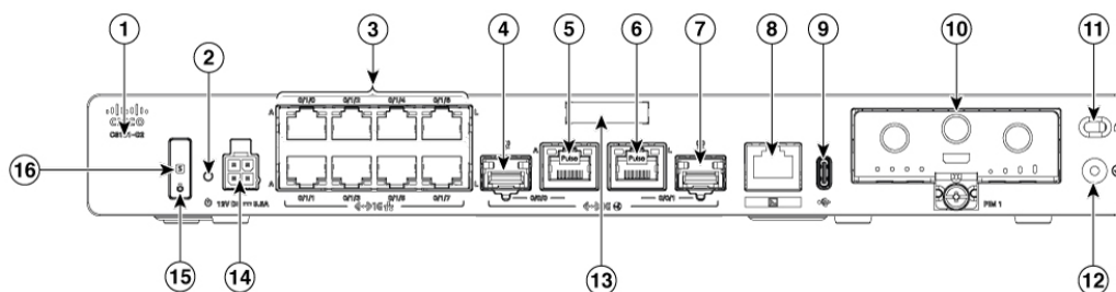
Figure 8: C8151-G2 - Front view
