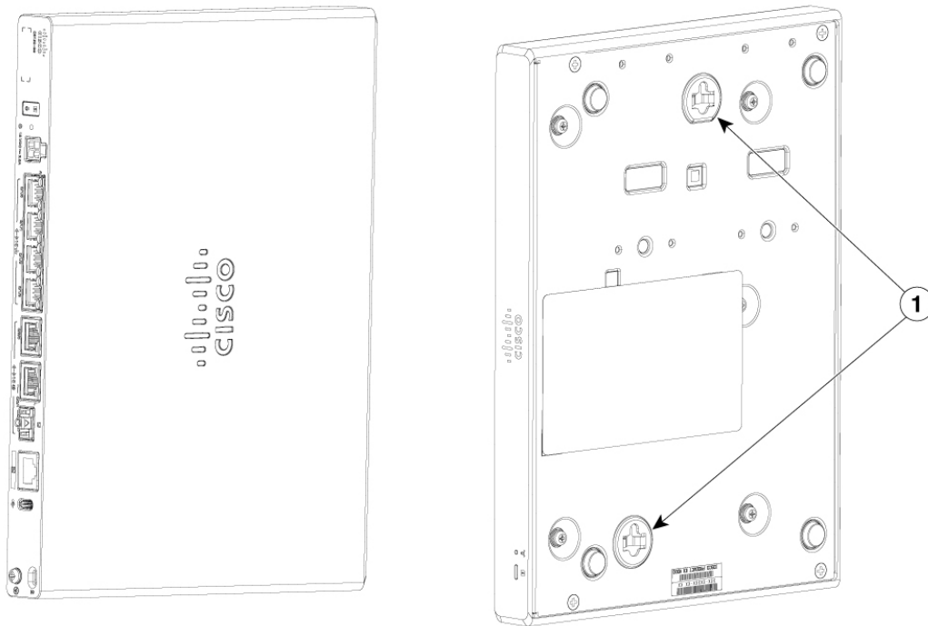
Figure 49: Wall mount using keyhole slots for C8130-G2 and C8131-G2
