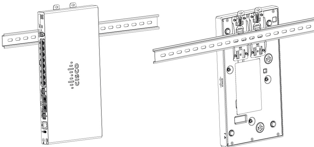
Figure 66: Mounting C8151-G2 and C8161-G2 using DIN rail brackets
