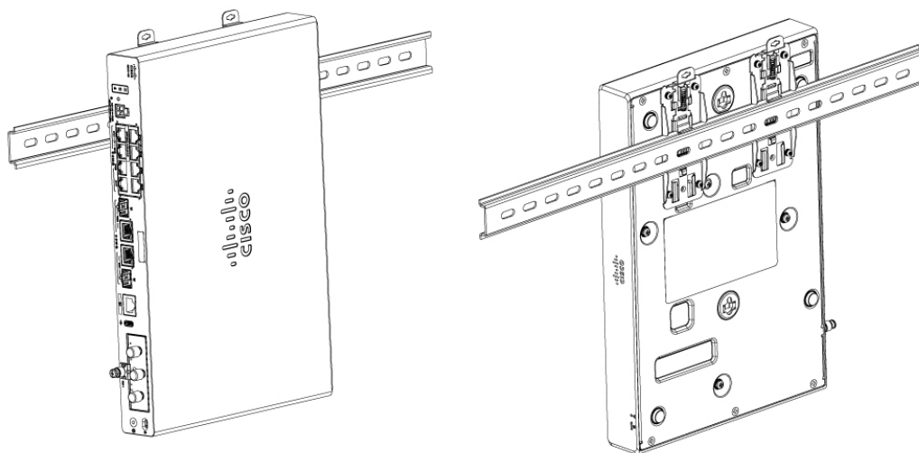
Figure 67: Mounting C8130-VAI-G2 and C8130-VAP-G2 using DIN rail brackets
