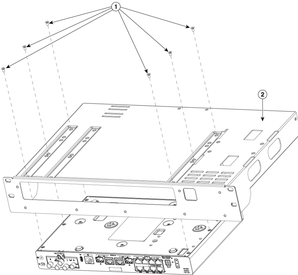
Figure 25: Rack mounting bracket installation for C8151-G2 and C8161-G2
