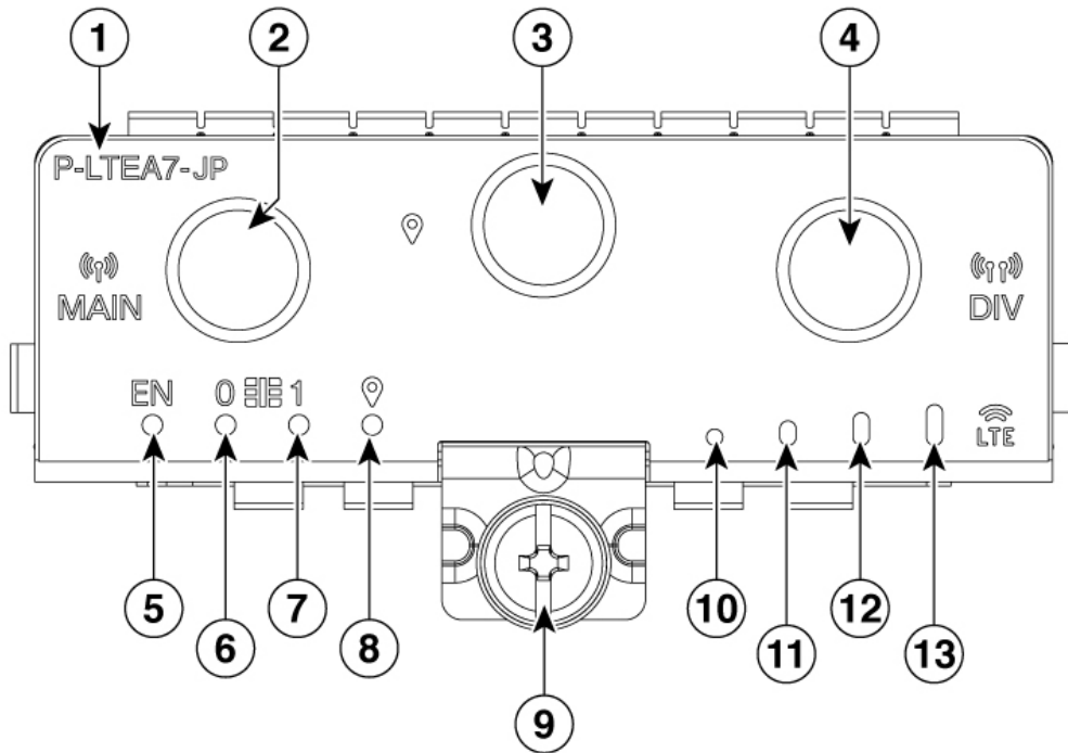
Figure 82: LTE Pluggable Interface Module - P-LTEA7-JP
