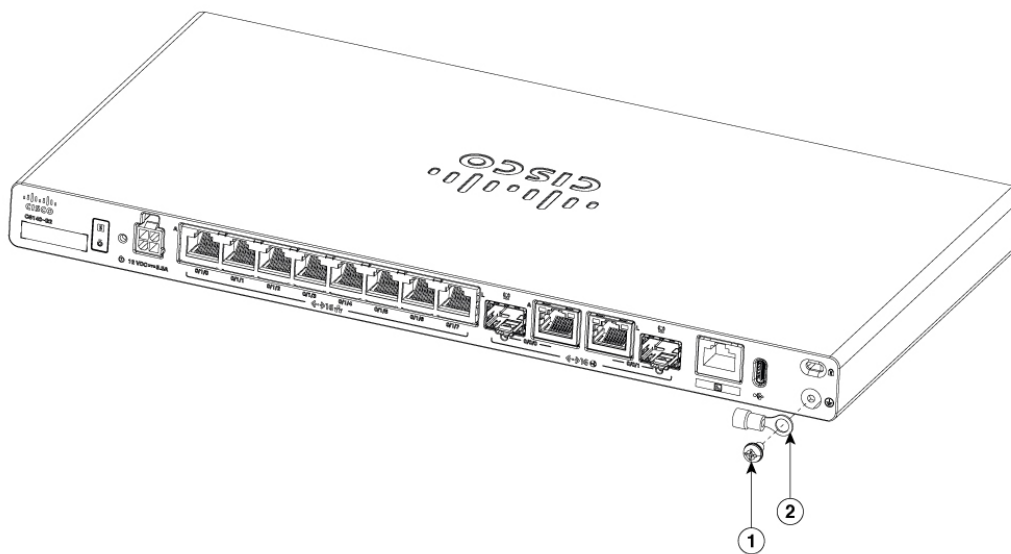
Figure 70: Chassis ground connection - C8140-G2
