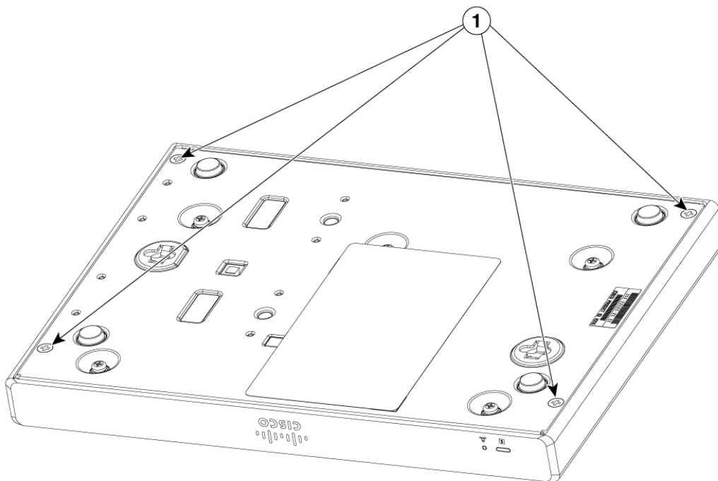
Figure 28: Removing screws from C8130-G2 and C8131-G2
