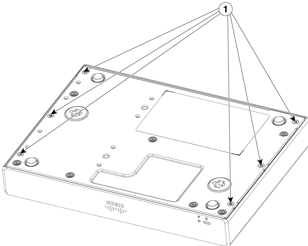
Figure 22: Removing screws from C8151-CVAI-G2 and C8151-CVAP-G2
