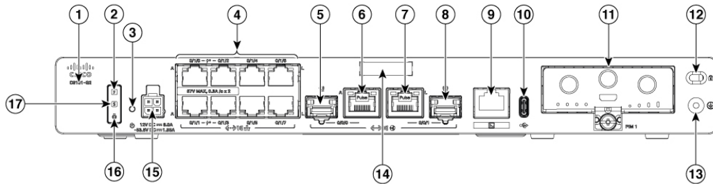
Figure 10: C8161-G2 - Front view
