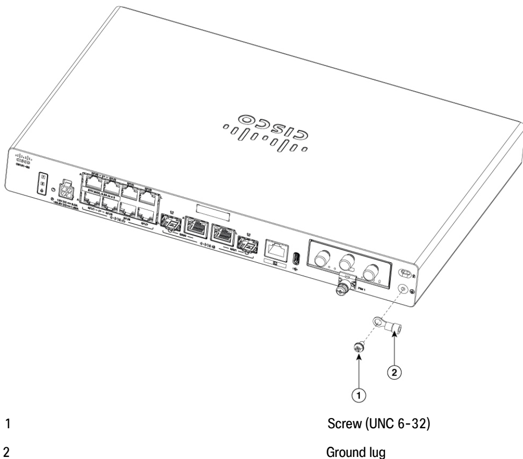
Figure 72: Chassis ground connection - C8130-VAI-G2 and C8130-VAP-G2
