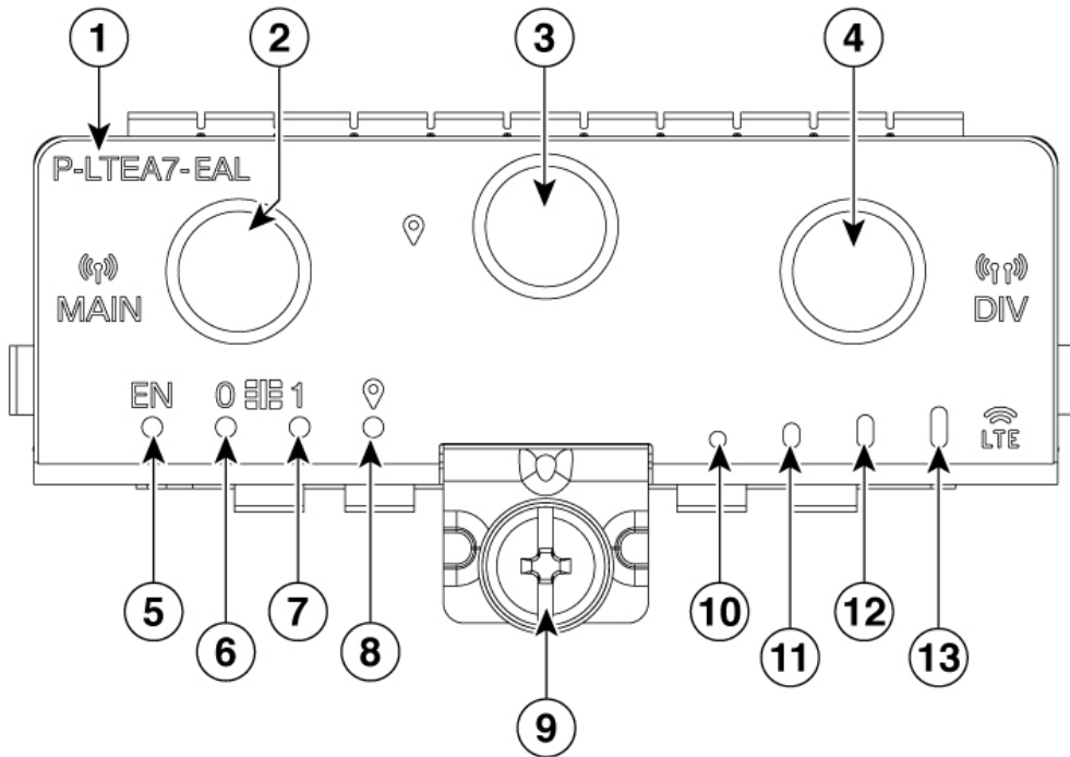
Figure 81: LTE Pluggable Interface Module - P-LTEA7-EAL
