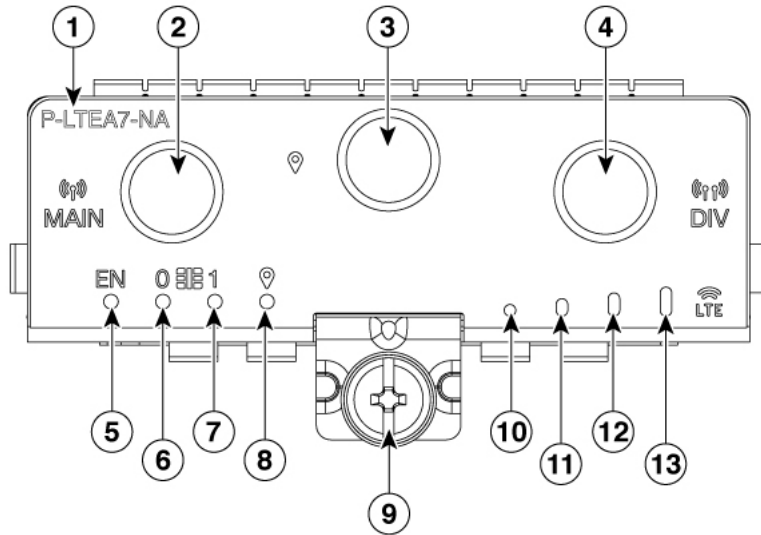
Figure 83: LTE Pluggable Interface Module - P-LTEA7-NA
