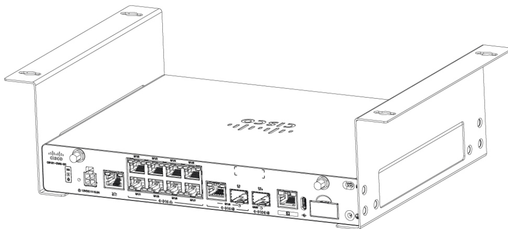
Figure 42: C8151-CVAI-G2 and C8151-CVAP-G2 with attached under desk mounting brackets
