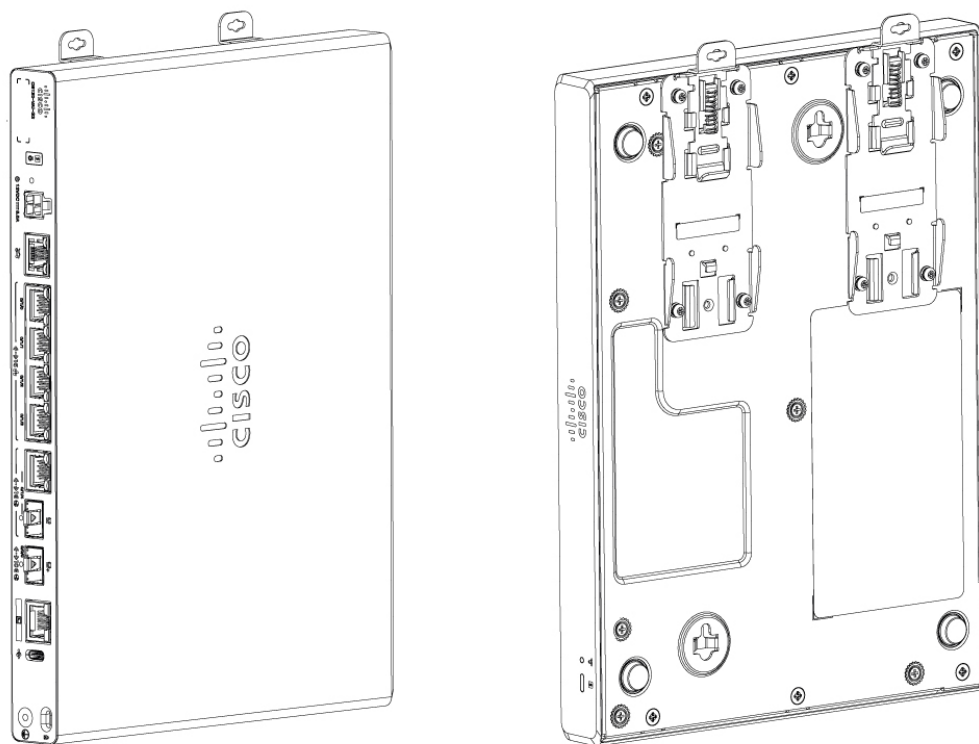
Figure 63: C8151-CVAI-G2 and C8151-CVAP-G2 with attached DIN rail brackets
