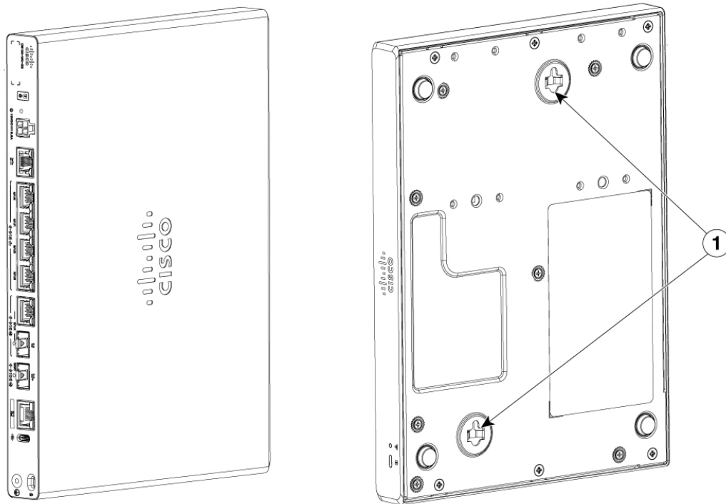
Figure 52: Wall mount using keyhole slots for C8130-VAI-G2 and C8130-VAP-G2
