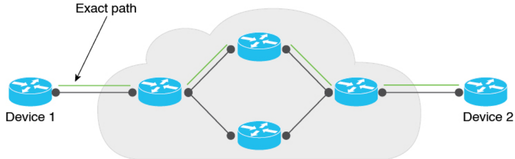
Figure 1: Exact Path
