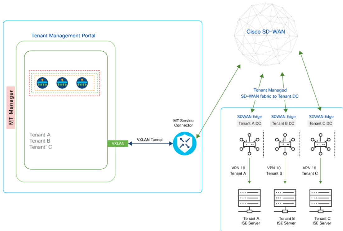
Figure 3: ISE integration for tenants
