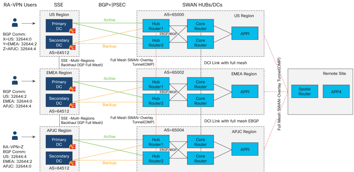
Figure 2: Example generic topology: SD-WAN hubs deployed in active/active model
