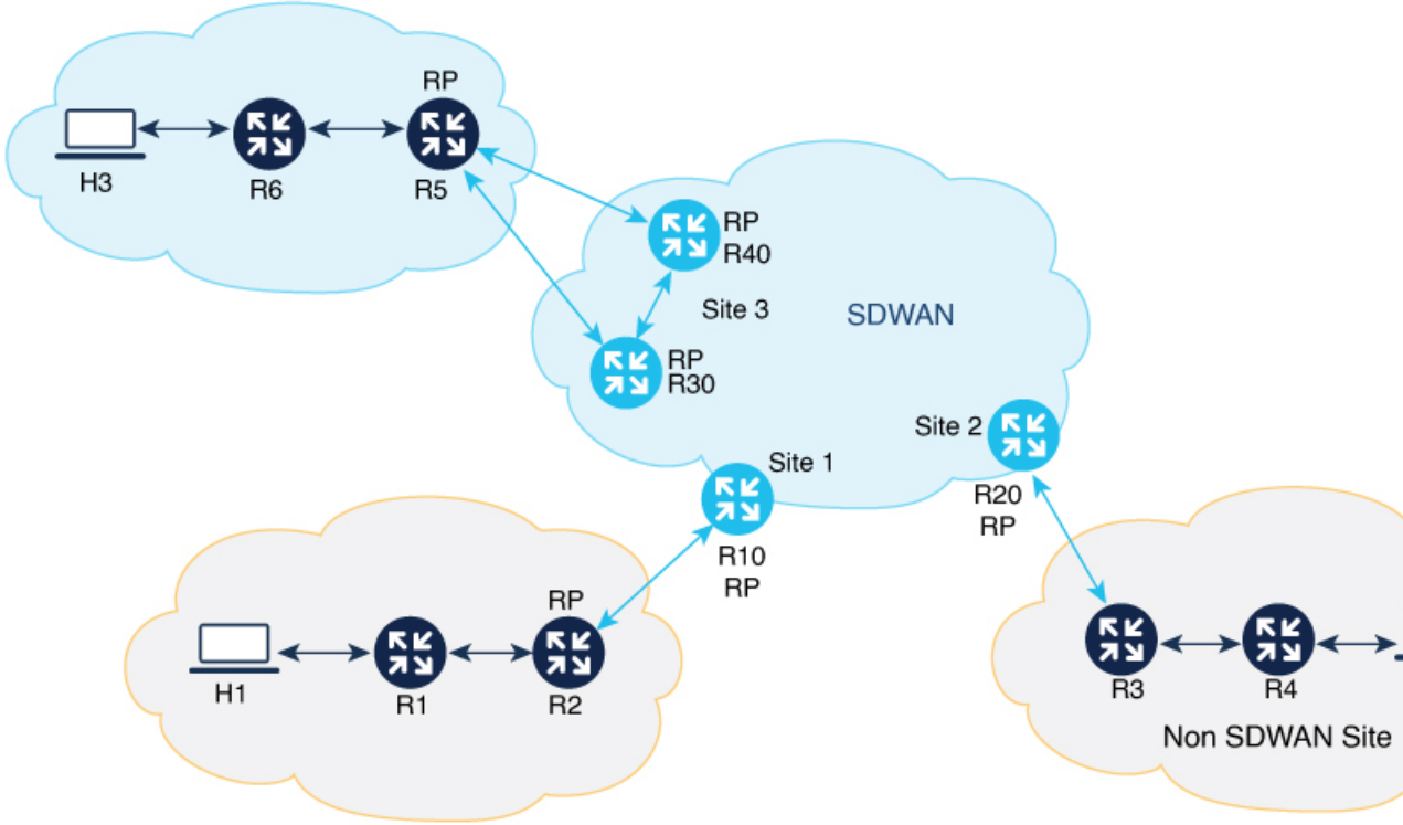
Figure 11: MSDP Interoperability
