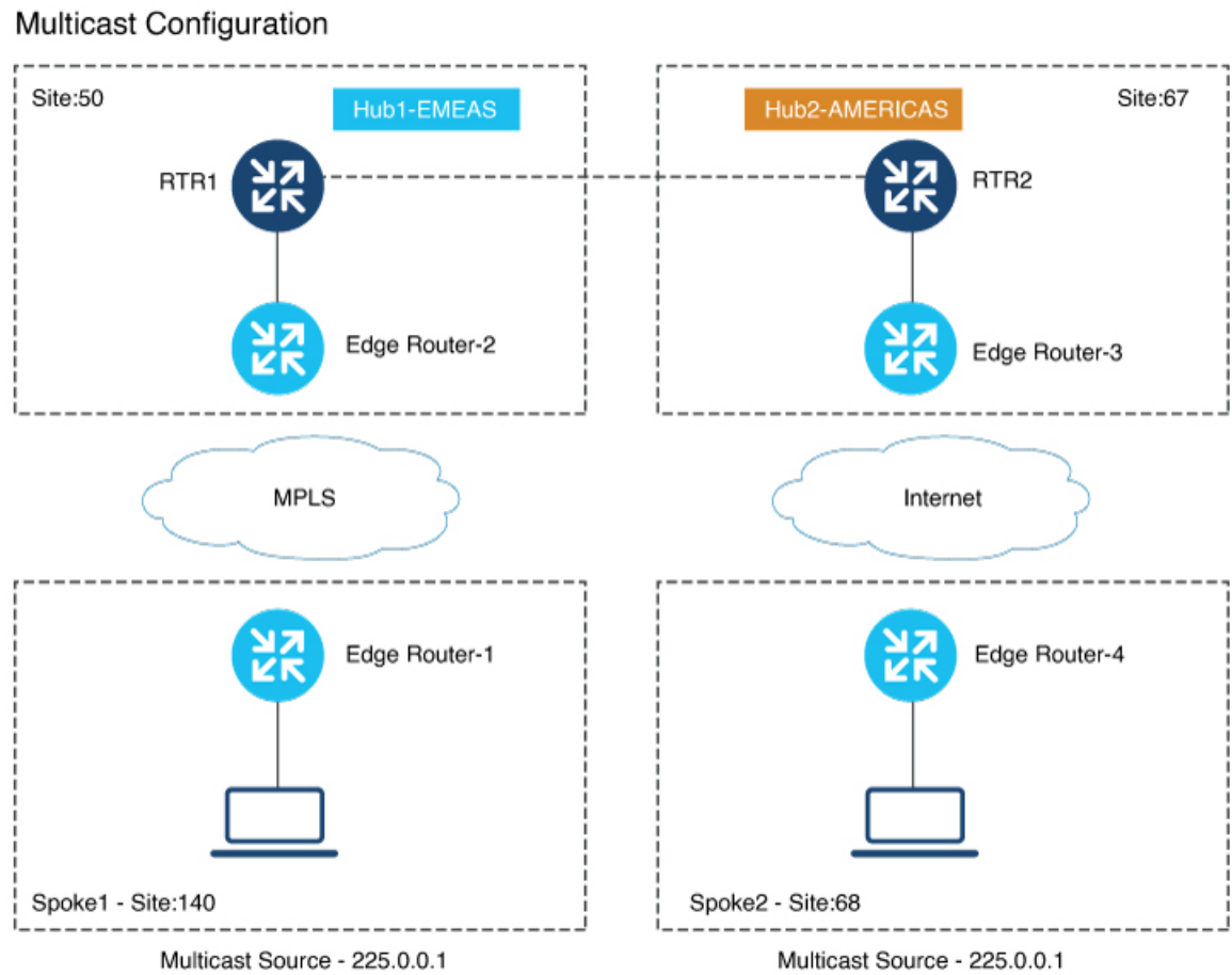
Figure 5: Multicast Configuration
