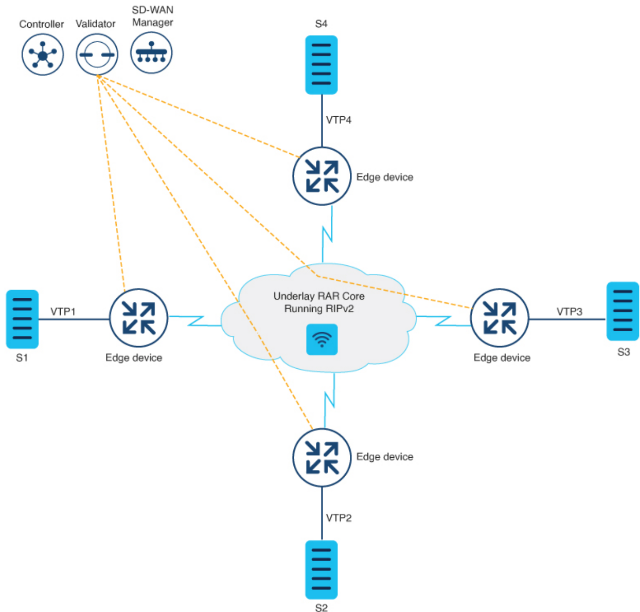
Figure 6: RAR architecture
