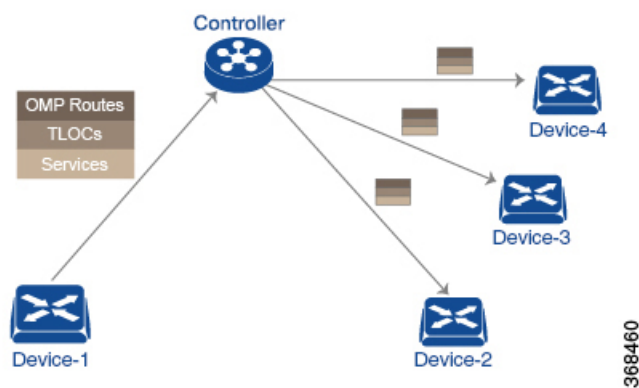
Figure 7: Control policy topology
