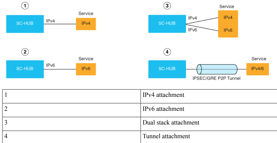
Figure 29: Attaching Services to a Router
