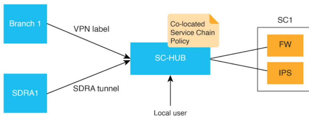
Figure 23: Traffic Steering with Traffic Service Chaining Intent Specified on a Local Device
