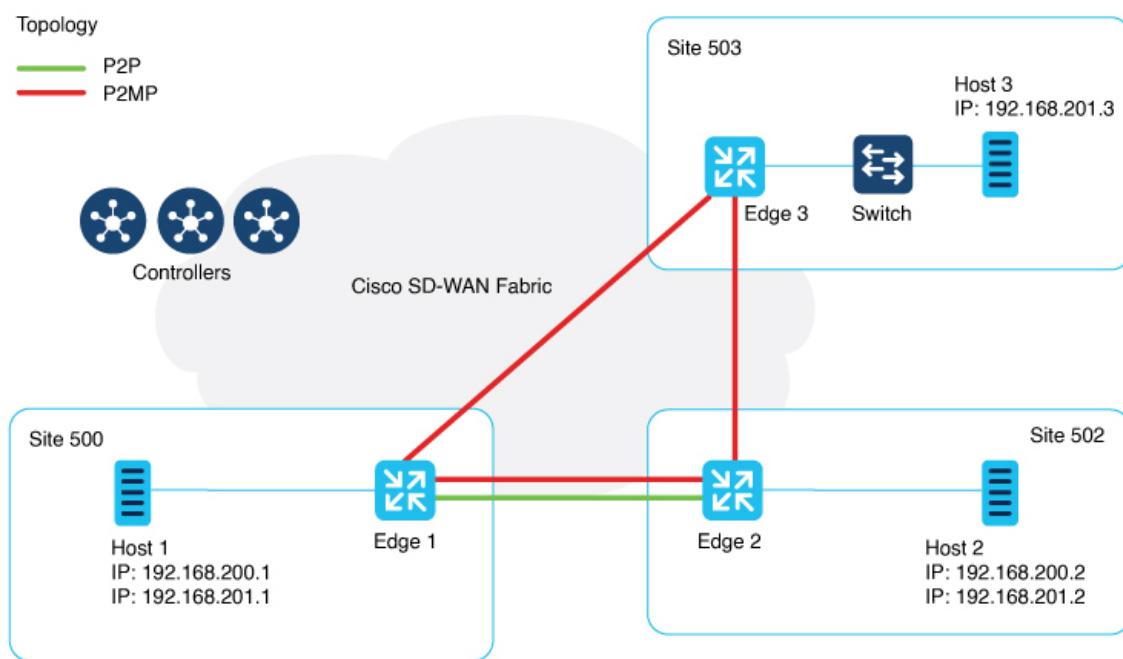
Figure 1: Topology
