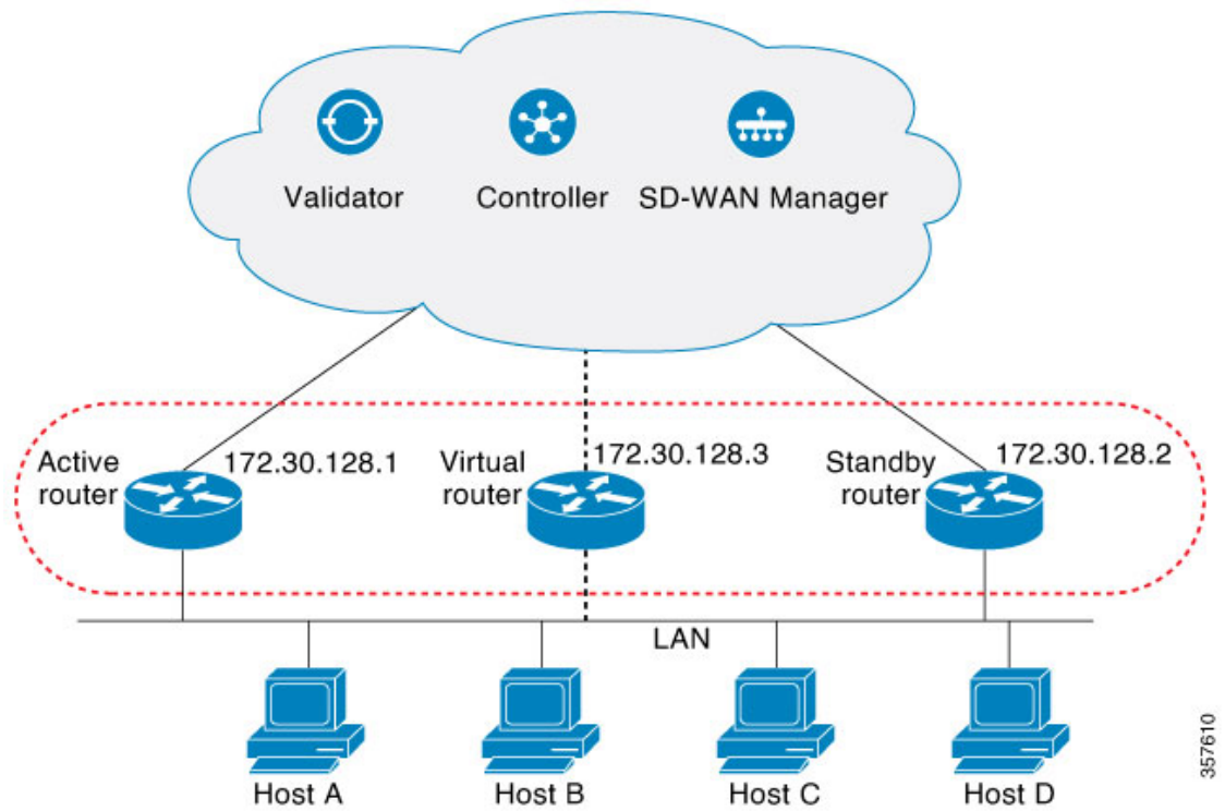
Figure 1: HSRP Topology
