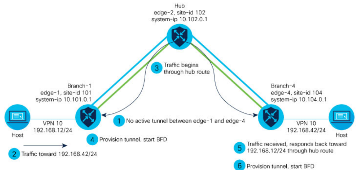
Figure 1: Process of On-Demand Tunnel Establishment Between Two Edge Routers
