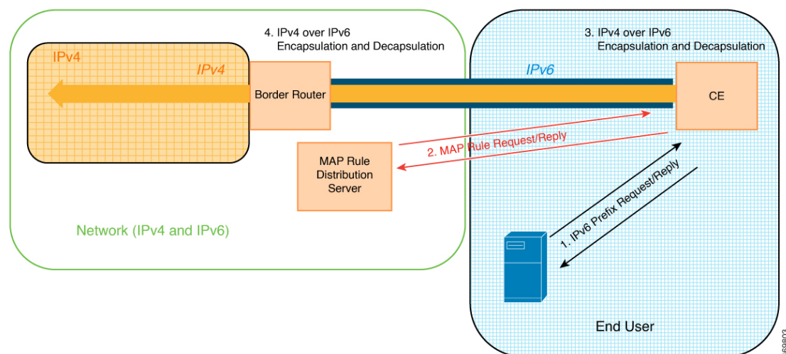
Figure 2: MAP-E Workflow
