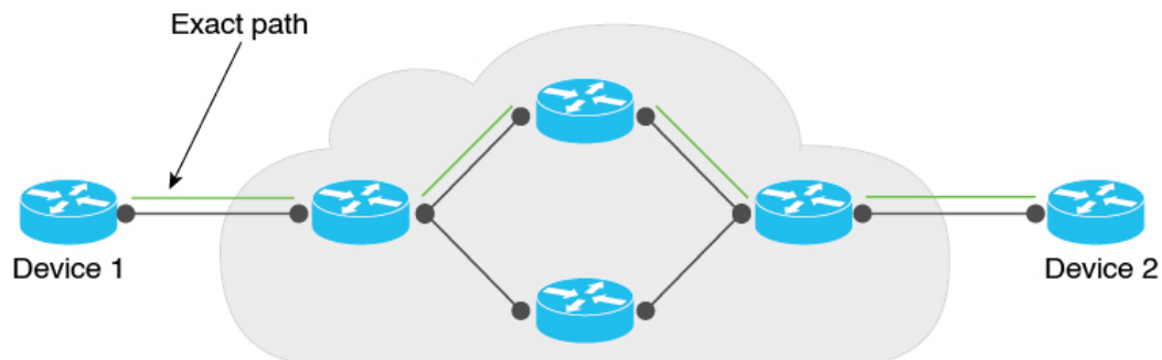
Figure 1: Exact Path
