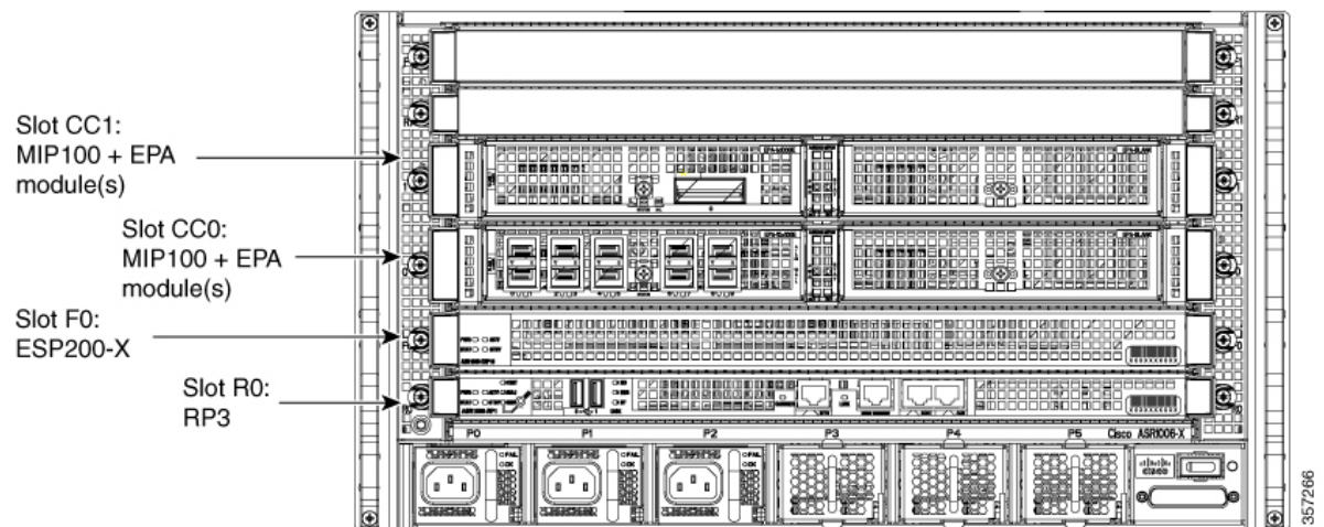
Figure 1: Cisco ASR 1006-X Slots and Modules
