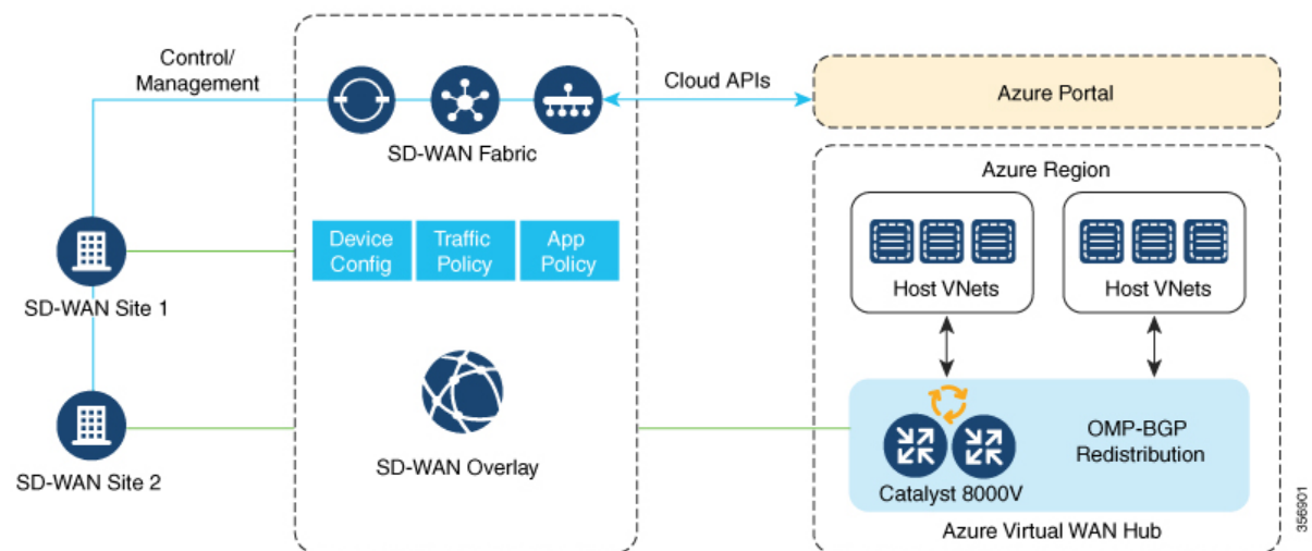
Figure 19: VNet to VNet Mapping within the Same Azure Region
