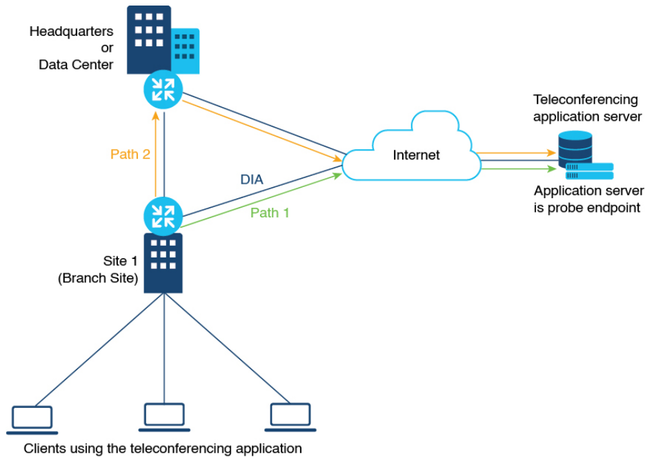
Figure 17: Use Case
