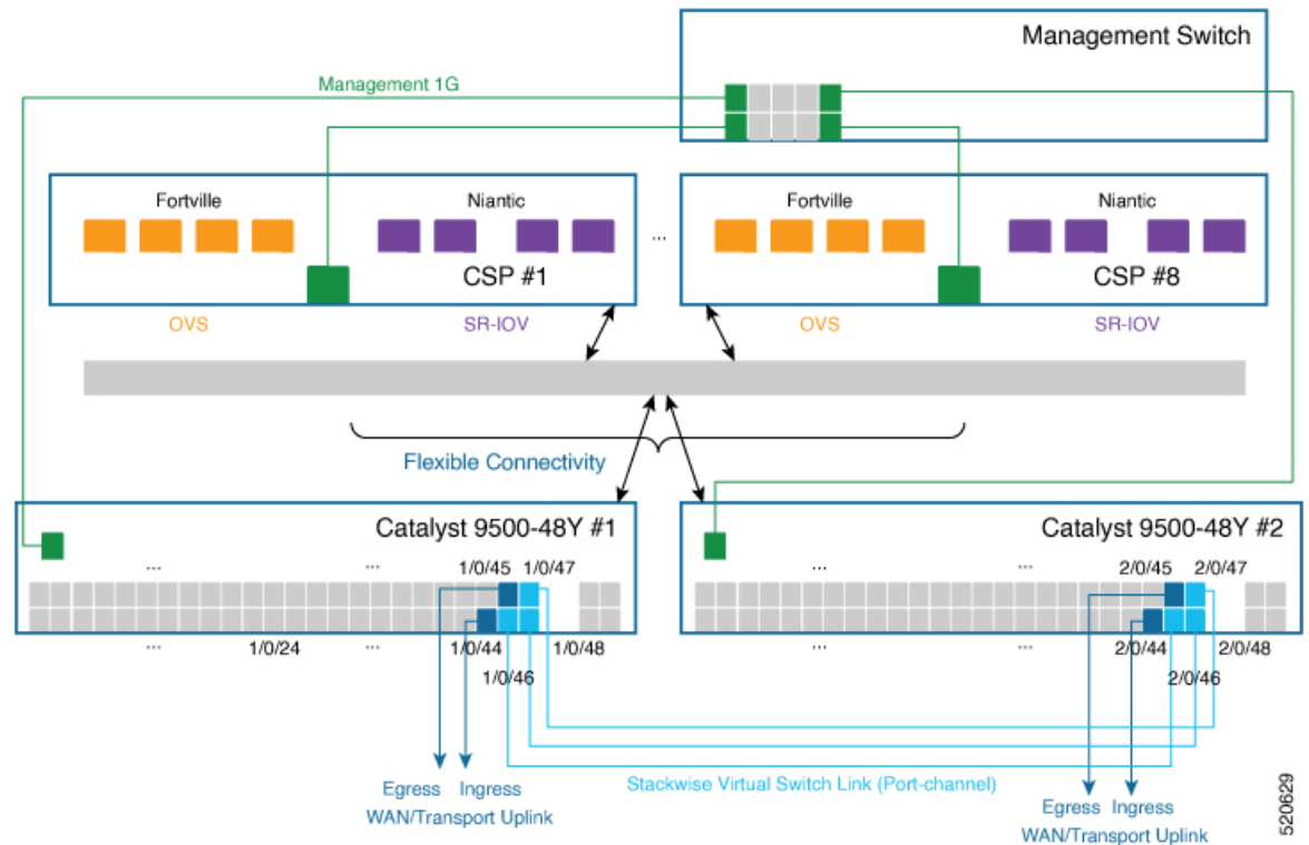
Figure 2: Cisco Catalyst SD-WAN Cloud OnRamp for Colocation Solution Flexible Connections
