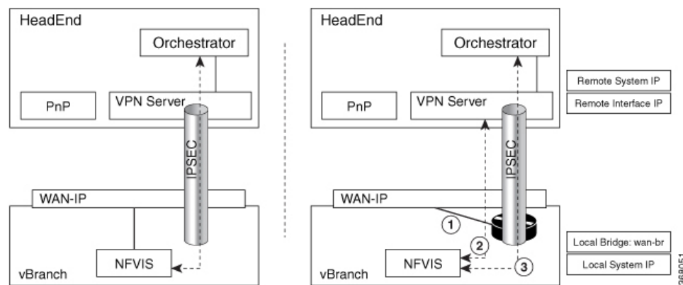
Figure 1: Example of Setting IPSec Tunnel in Single IP mode
