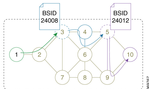
Figure 1: Intra-Domain Topology
