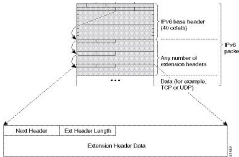
Figure 8: IPv6 Extension Header Format
