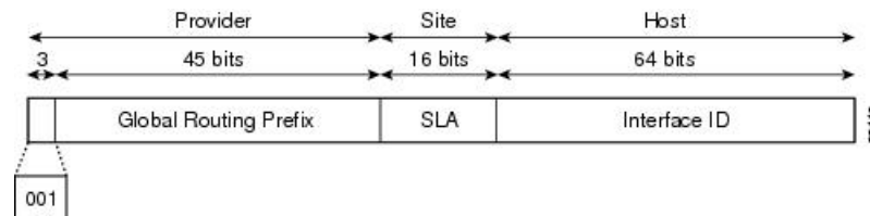
Figure 1: Aggregatable Global Address Format
