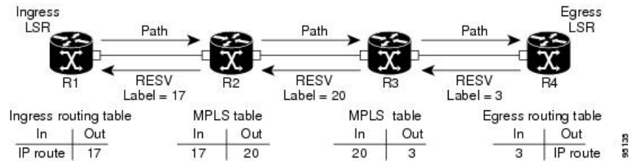
Figure 1: RSVP Operation
