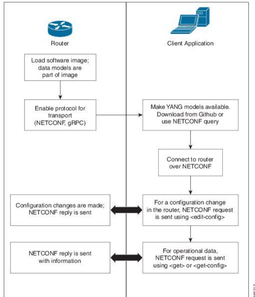
Figure 1: Process for Using Data Models
