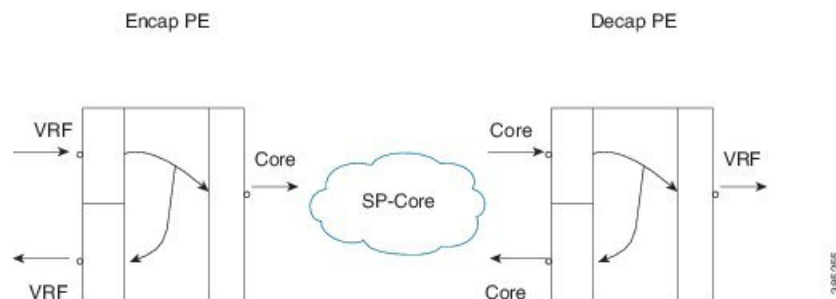
Figure 8: Forwarding Scheme
