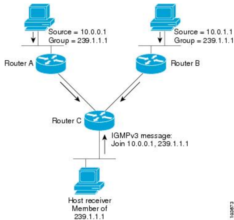
Figure 5: Designated Router Election on a Multiaccess Segment
