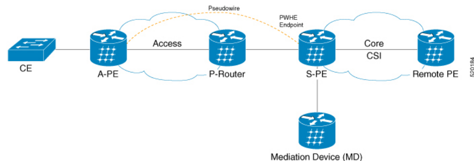
Figure 4: Lawful Intercept
