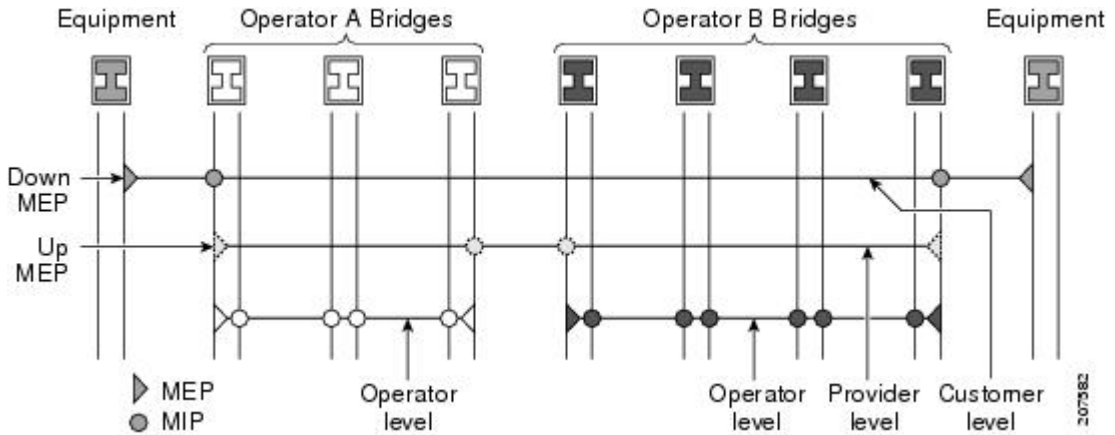
Figure 5: Data CFM Maintenance Points at Different Levels
