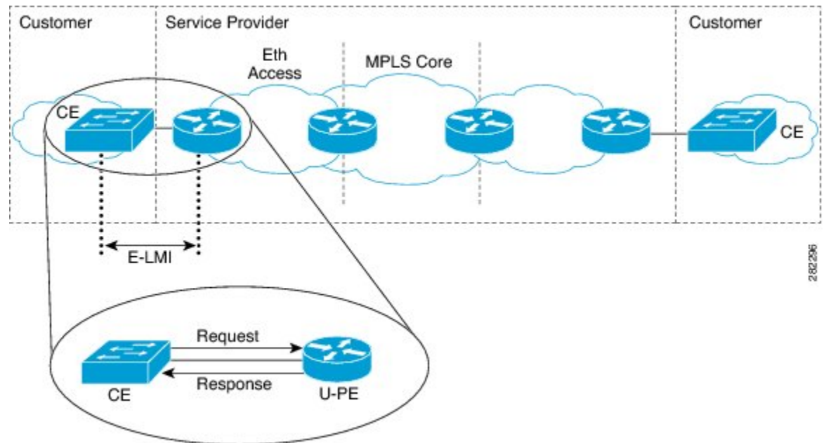
Figure 13: E-LMI Communication on CE-to-PE Link
