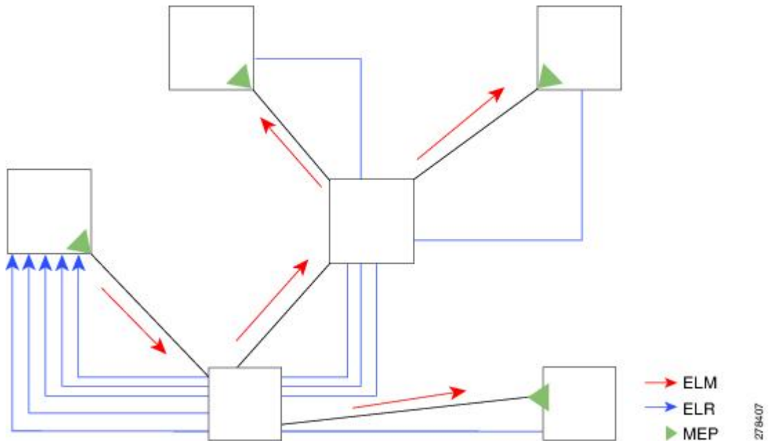
Figure 9: Exploratory Linktrace Messages and Replies
