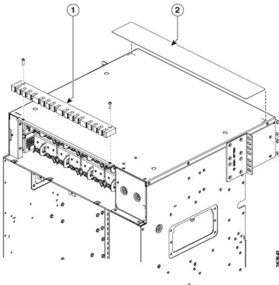
Figure 14: Attaching Rear Cable Guide and Insulator Sheet
