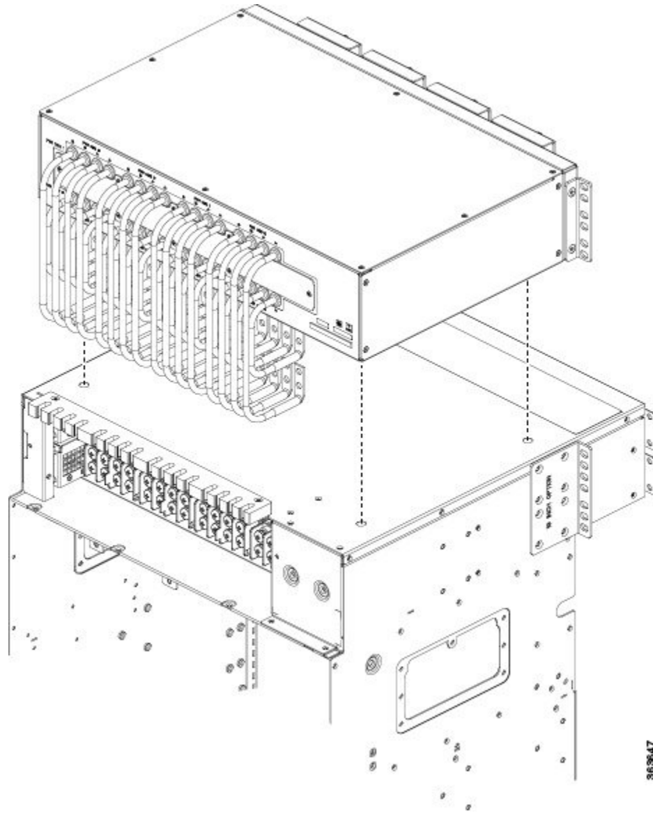
Figure 15: Placing DC Adapter on Top of Chassis
