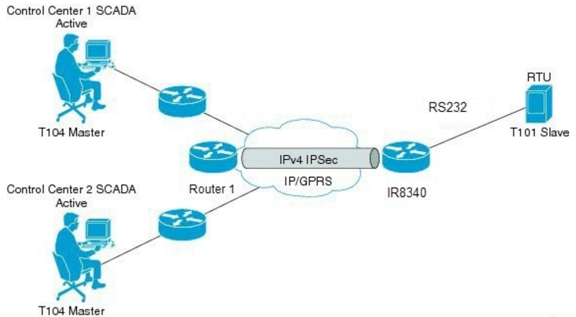
Figure 2: Routers Within a SCADA System
