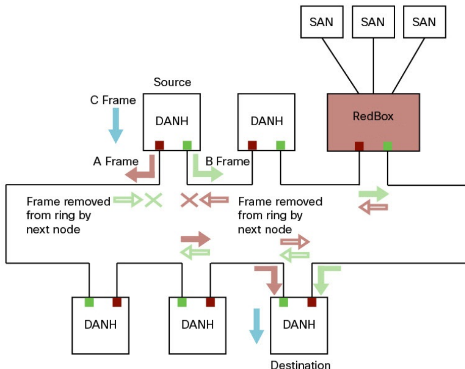
Figure 3: Example of HSR Ring Carrying Unicast Traffic
