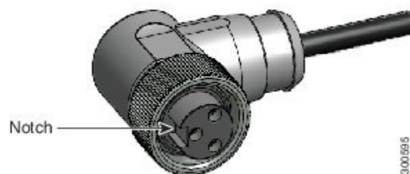
Figure 1: Router AC Power Cable (Router Connector End)
