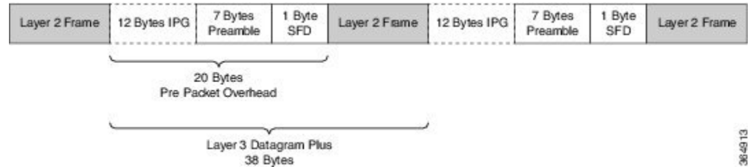
Figure 5: Ethernet Overhead
