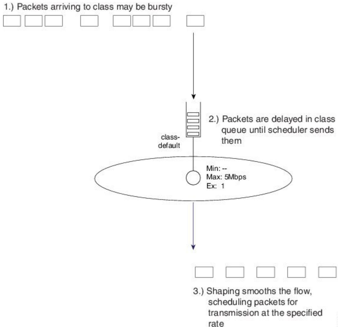
Figure 11: Single-shaped Queue
