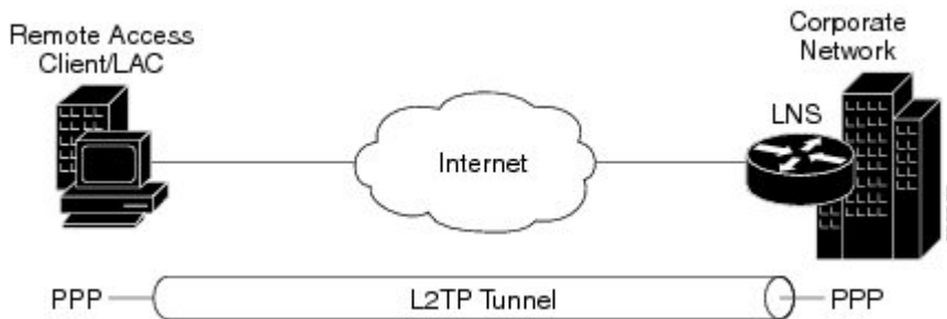
Figure 6: L2TPv2 Tunnel to an LNS Device
