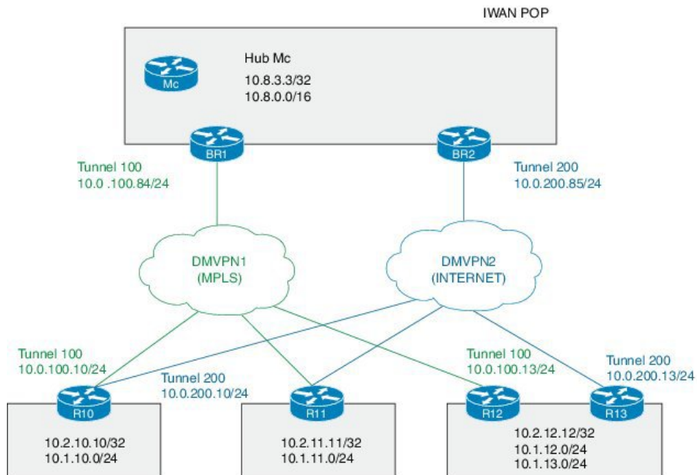
Figure 2: PfRv3 Topology
