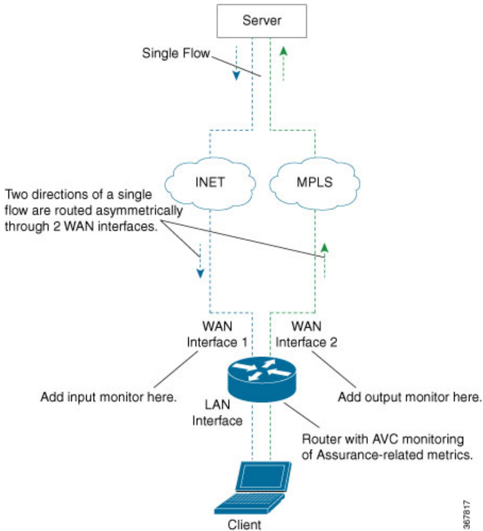
Figure 13: Asymmetric Routing
