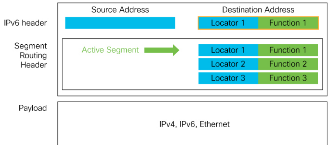
Figure 1: Network Program in the Packet Header
