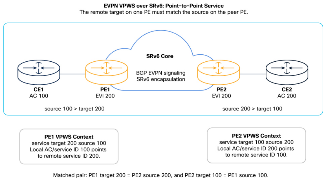
Figure 4: EVPN VPWS over SRv6 point-to-point service
