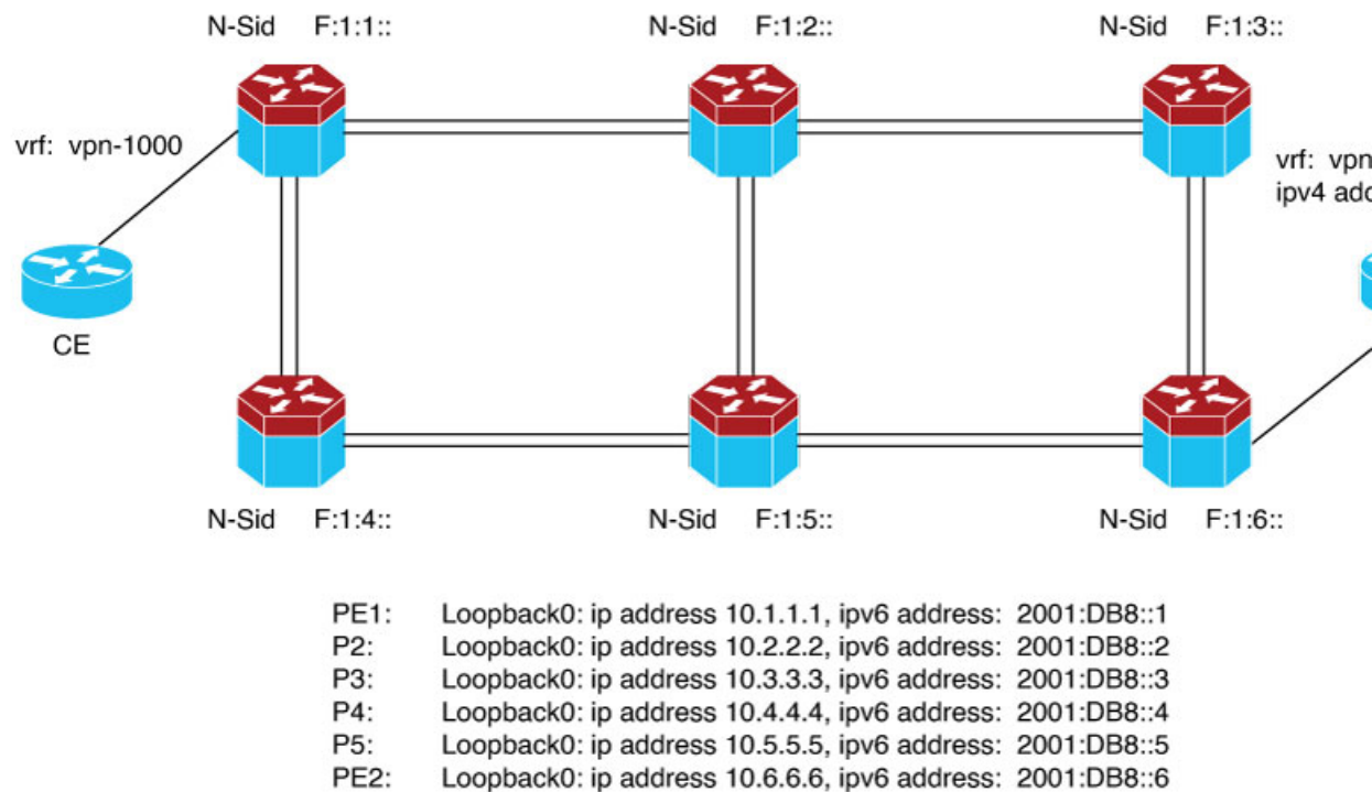
Figure 6: SRv6 OAM Topology
