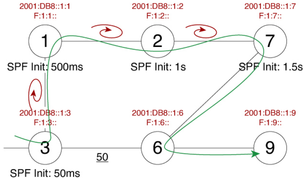
Figure 49: Microloop Example Topology—Microloops
