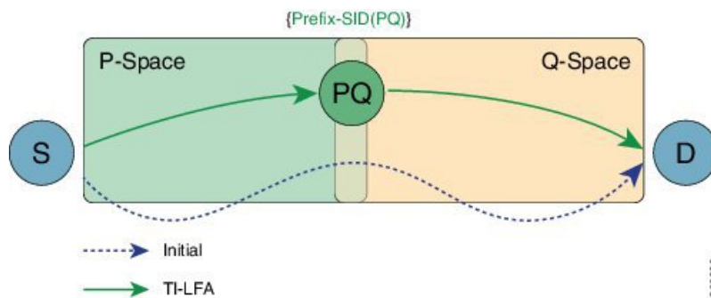
Figure 7: TI-LFA: { Prefix-SID(PQ) }
