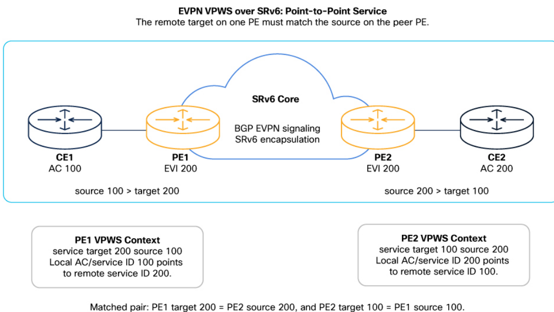
Figure 43: EVPN VPWS over SRv6 point-to-point service
