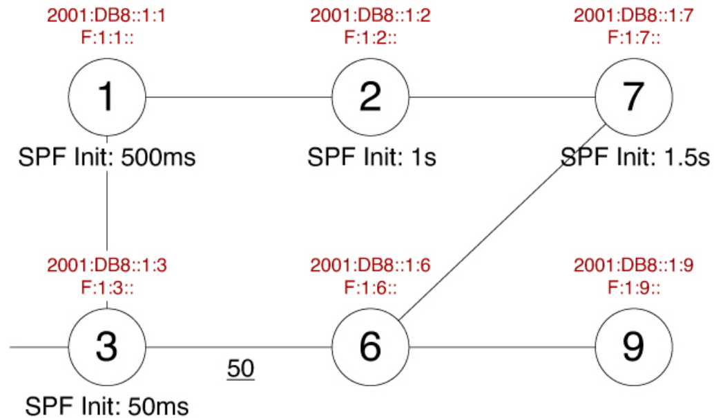
Figure 50: Microloop Example Topology—Segment Routing
