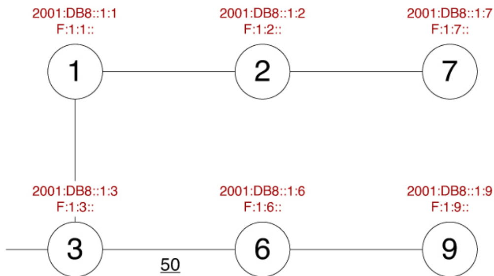
Figure 46: Microloop Example Topology
