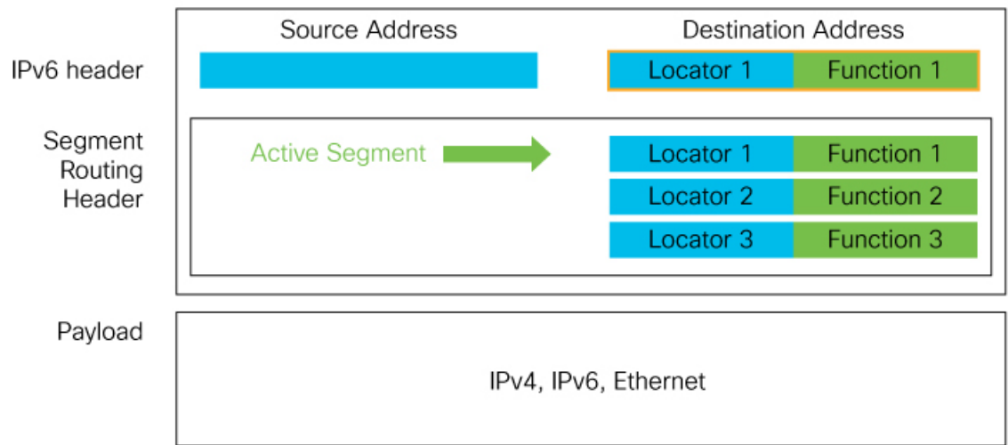
Figure 40: Network Program in the Packet Header
