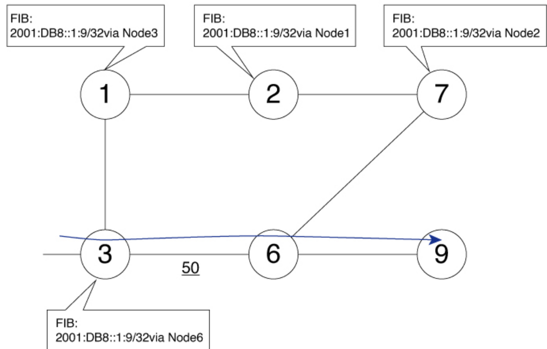
Figure 48: Microloop Example Topology—FIB Entry
