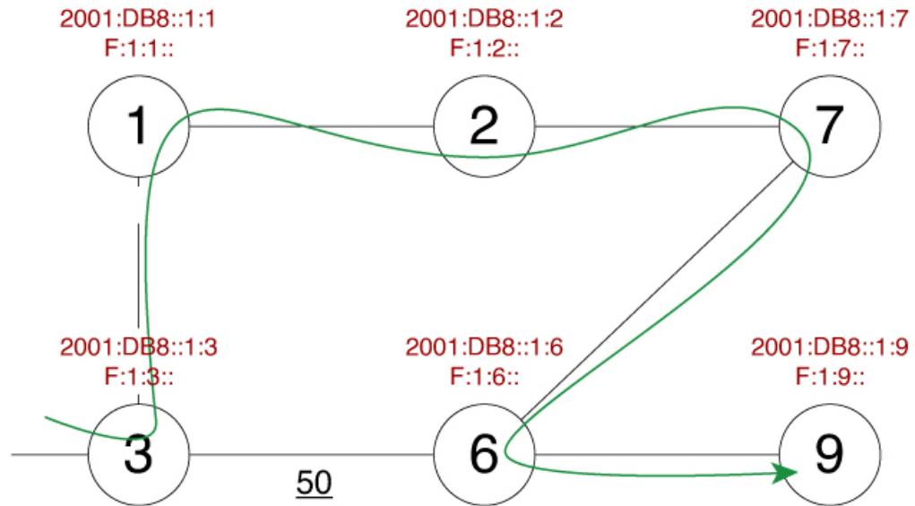
Figure 47: Microloop Example Topology—Shortest Path
