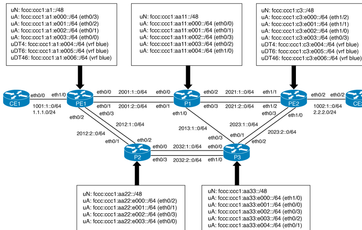
Figure 44: Sample SRv6 OAM Topology
