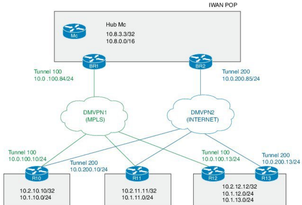
Figure 2: PfRv3 Topology
