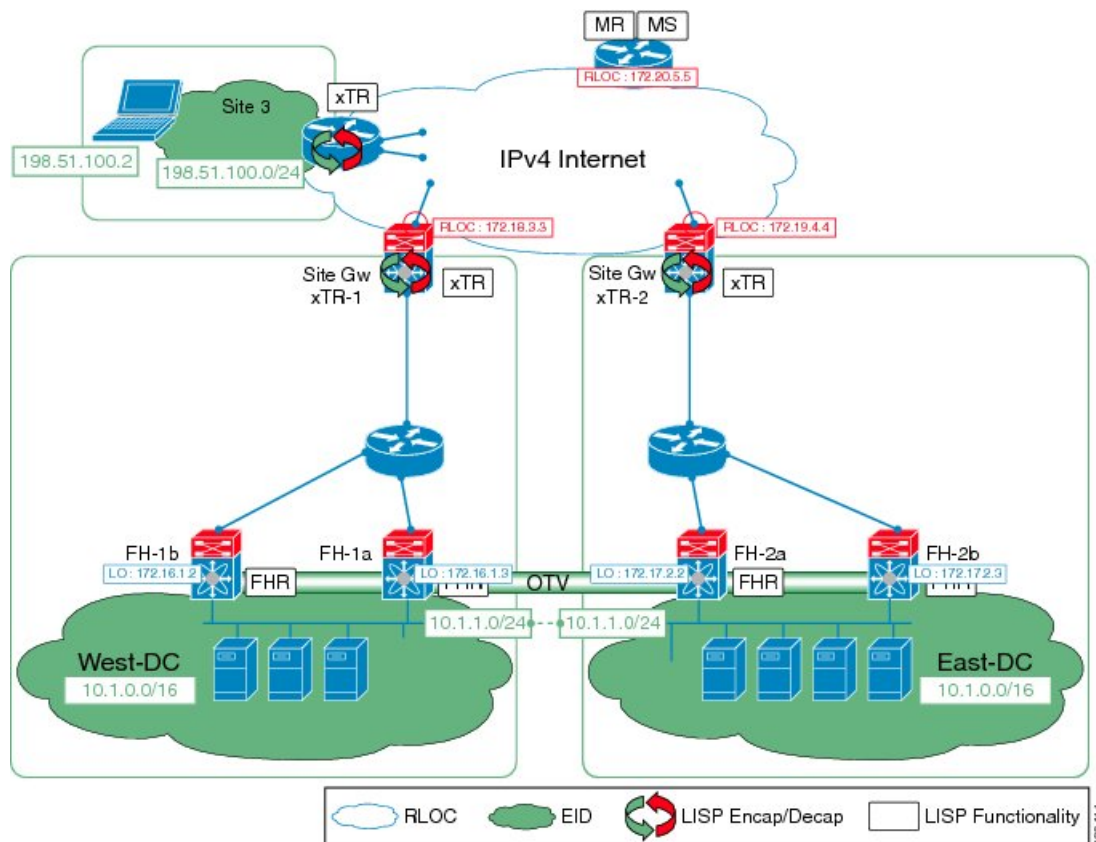
Figure 3: LISP ESM Multihop Topology
