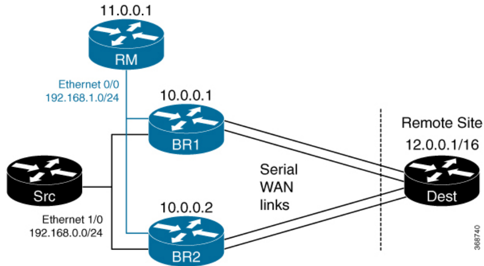
Figure 9: DAPR Topology
