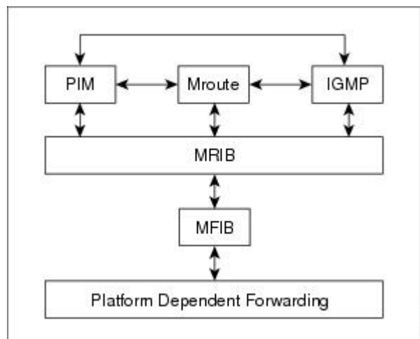
Figure 25: IPv4 MFIB Architecture
