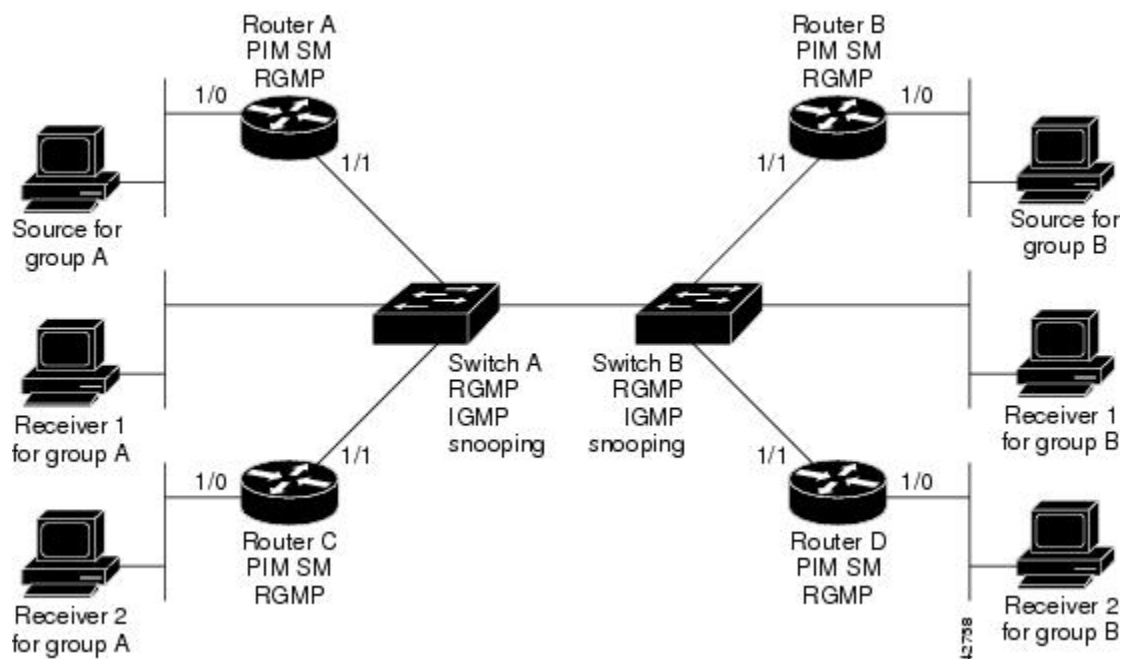
Figure 58: RGMP Configuration Example
