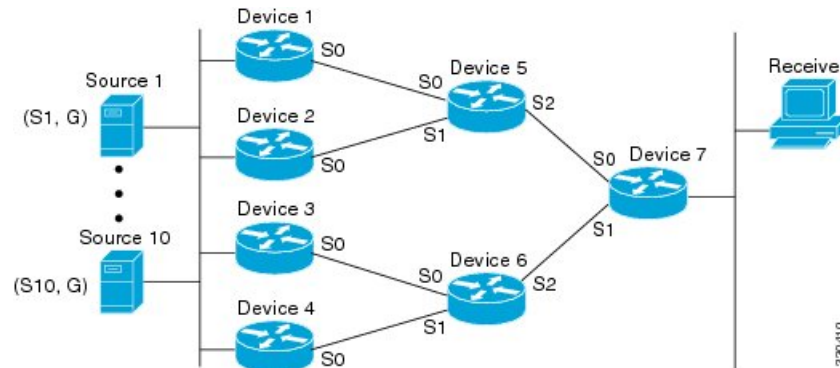
Figure 63: Polarization Topology
