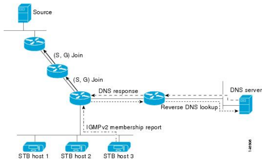
Figure 53: DNS-Based SSM-Mapping
