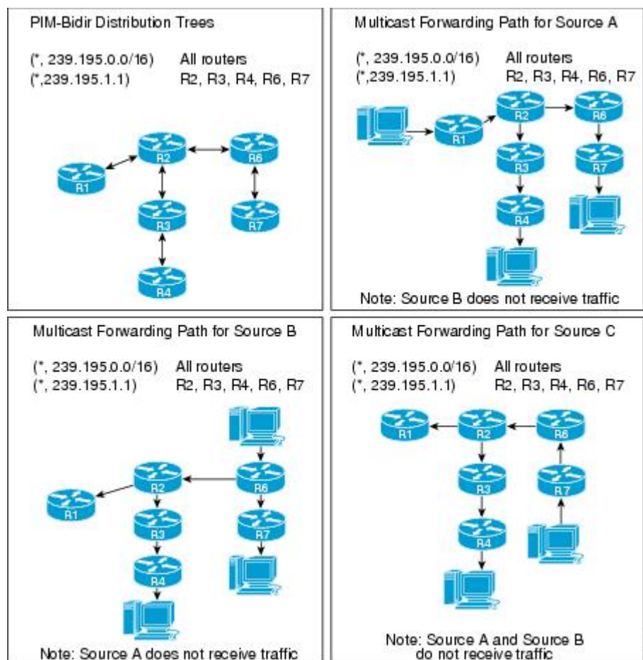
Figure 36: Bidir-PIM Distribution Trees and Multicast Forwarding Paths for the Active Sources with No Interested Receivers Example
