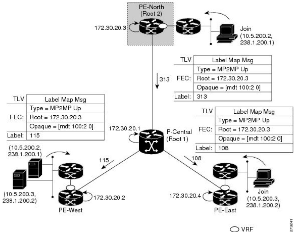
Figure 47: Default MDT Upstream--Root 2
