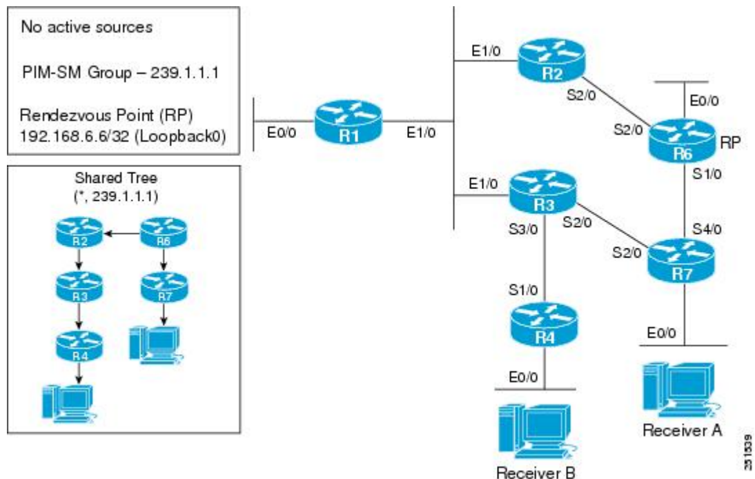
Figure 31: PIM-SM Example Topology: Interested Receivers with No Active Sources
