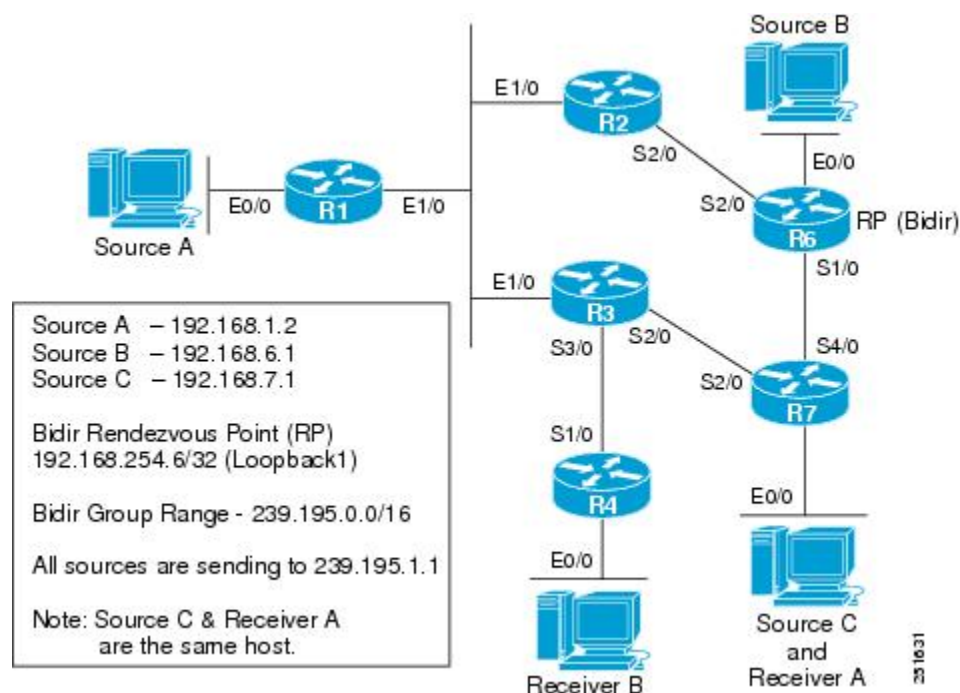
Figure 35: Bidir-PIM Example Topology: Active Sources with Interested Receivers
