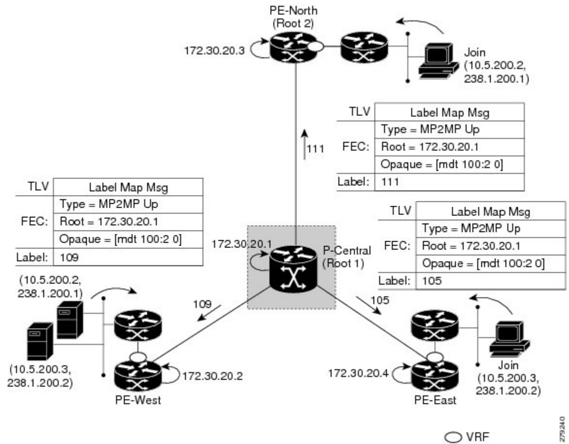
Figure 46: Default MDT Upstream--Root 1
