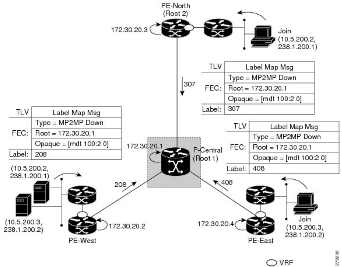
Figure 44: Default MDT Downstream--Root 1
