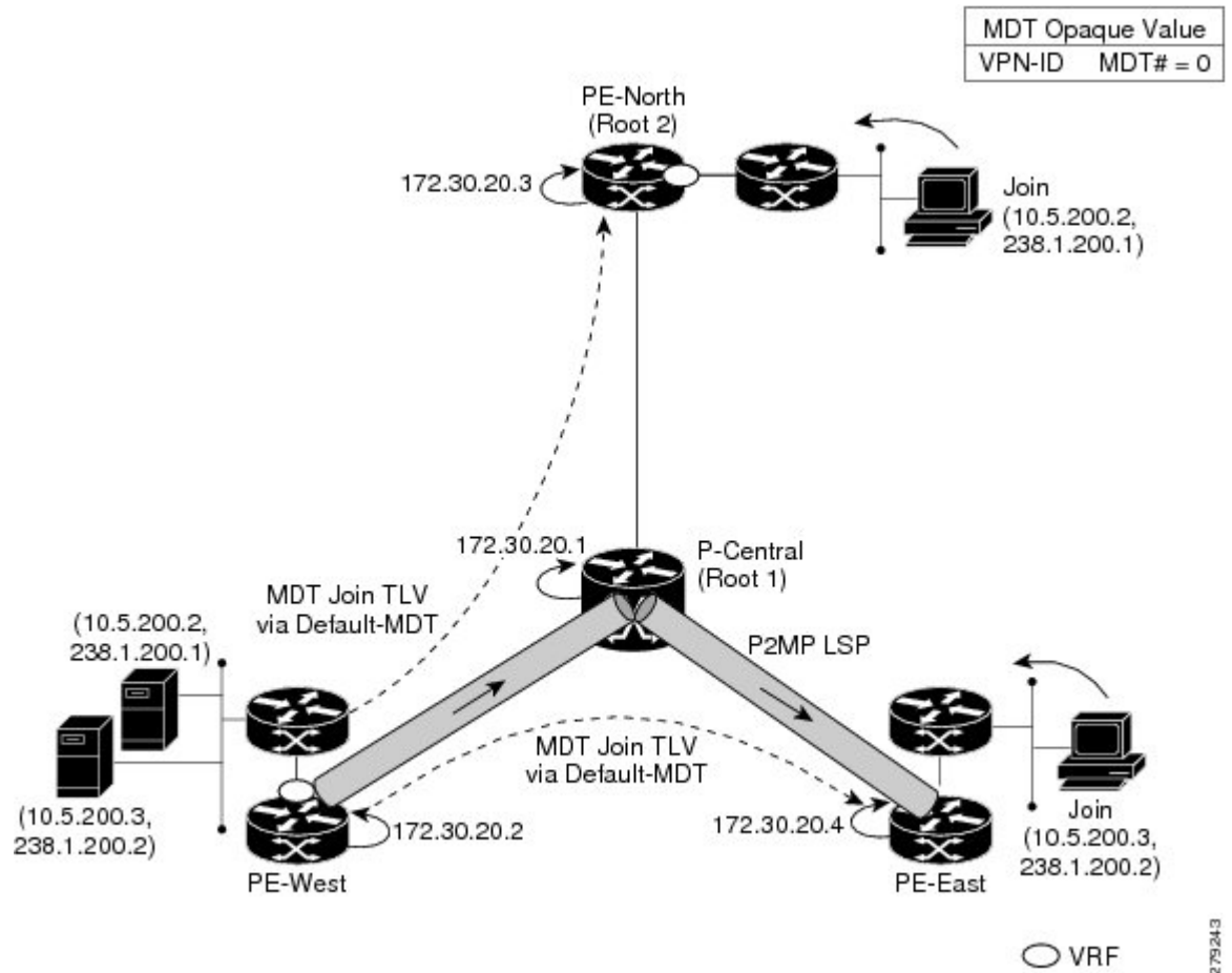
Figure 51: Data MDT Example
