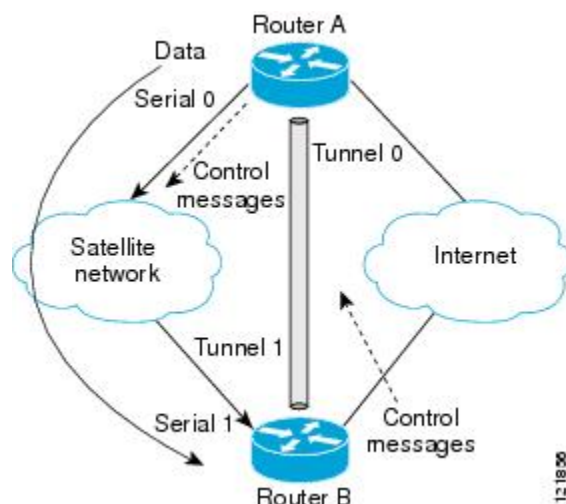
Figure 59: UDLR Tunnel Example
