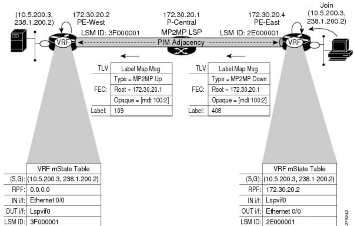
Figure 48: PIM Signaling over LSP
