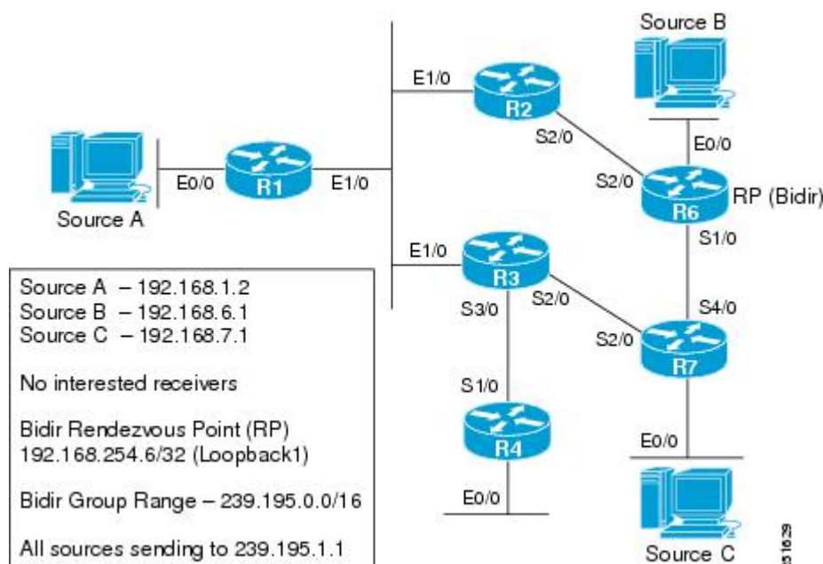
Figure 38: Bidir-PIM Distribution Trees and Multicast Forwarding Path for Active Sources with No Interested Receivers Example
