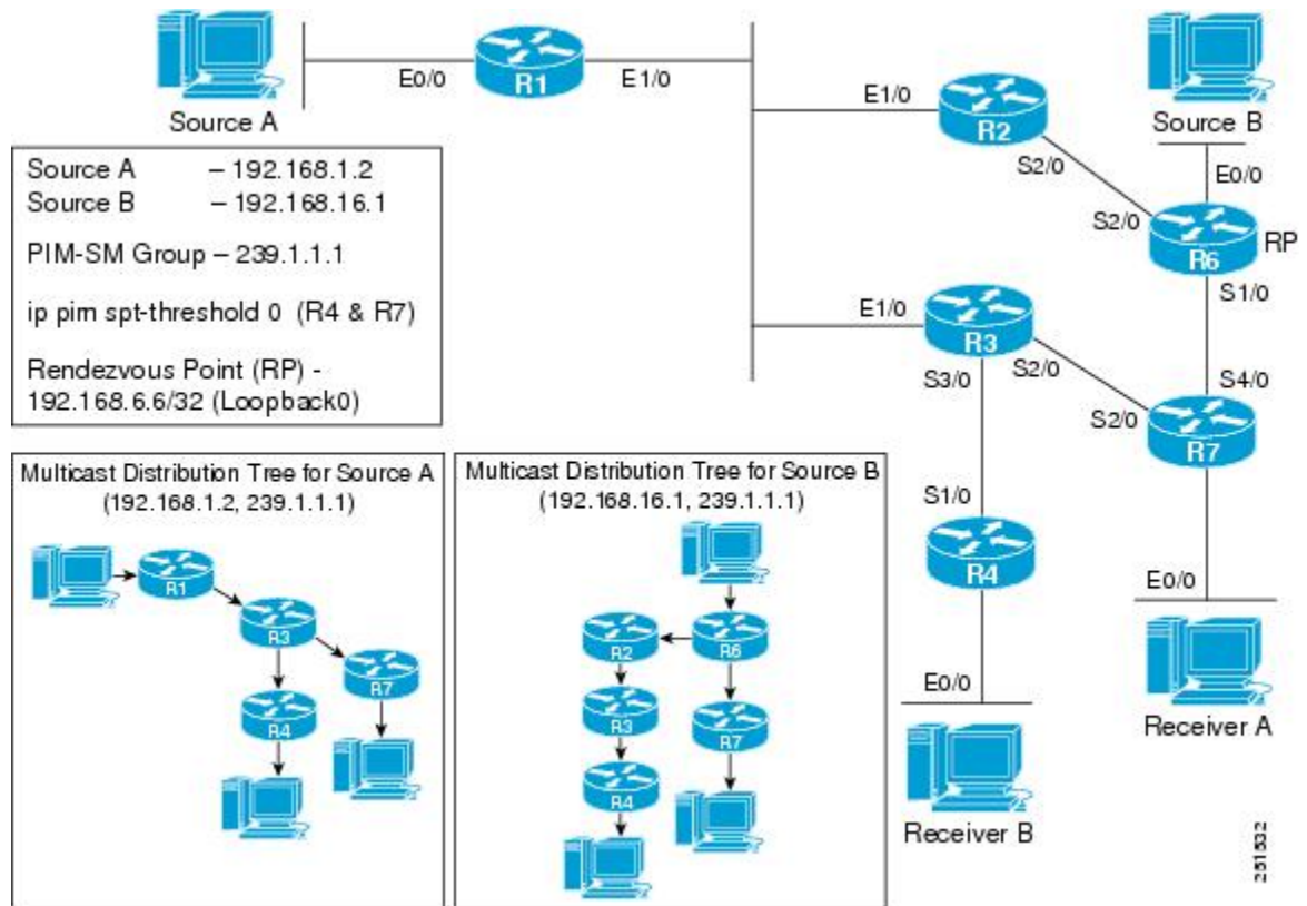
Figure 28: PIM-SM Example Topology: Active Sources and Interested Receivers (SPT Switchover)
