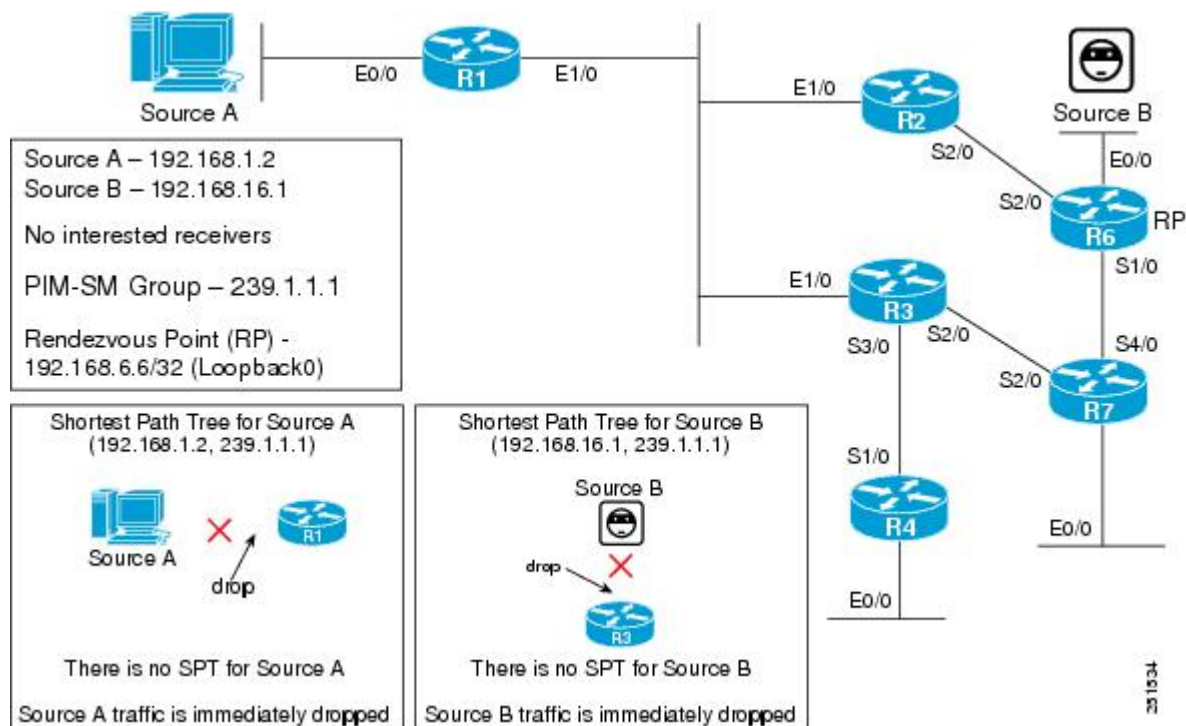
Figure 30: PIM-SM Example Topology: Source Traffic Only with No Receivers
