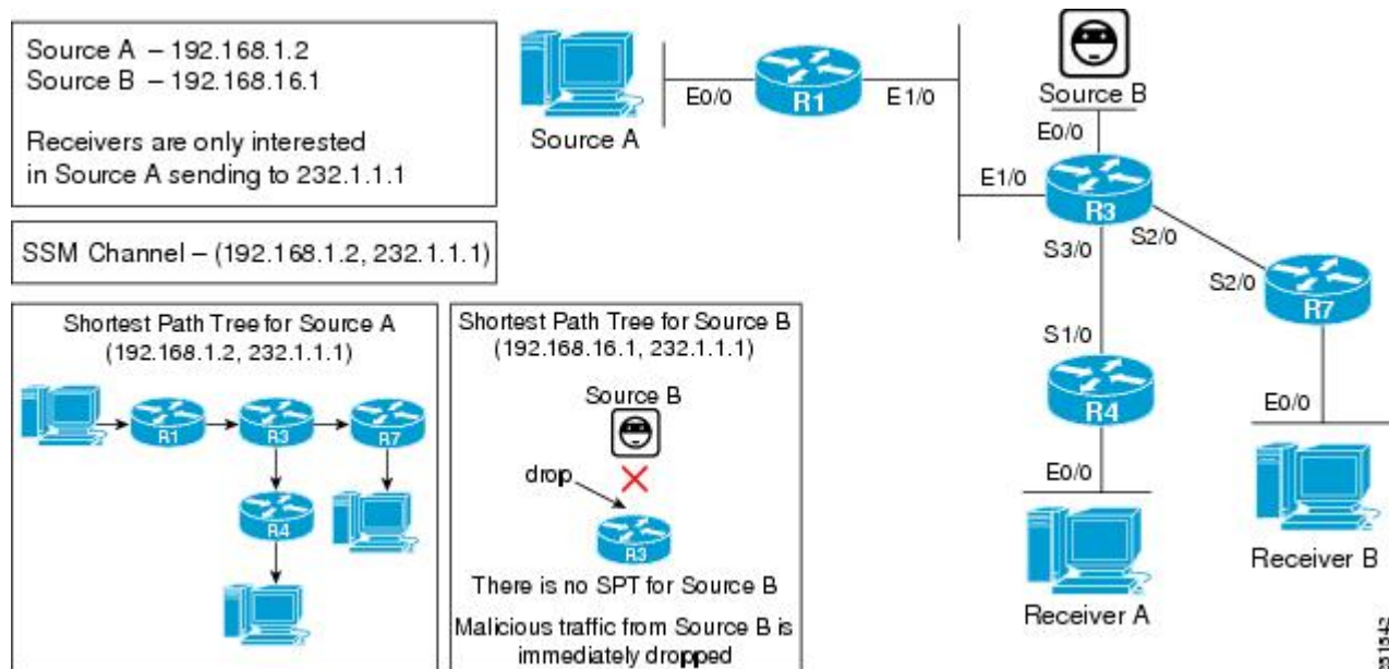
Figure 34: PIM-SSM Example Topology: Unwanted Sources in the SSM Network
