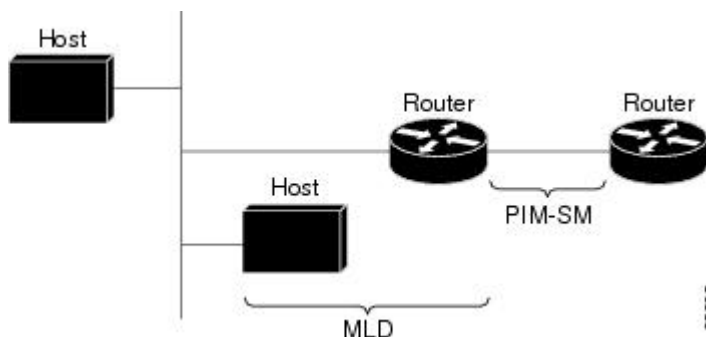
Figure 52: IPv6 Multicast Routing Protocols Supported for IPv6
