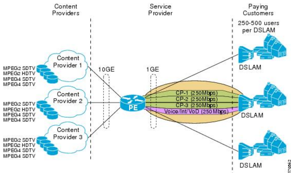
Figure 68: Bandwidth-Based CAC for IP Multicast Example Topology
