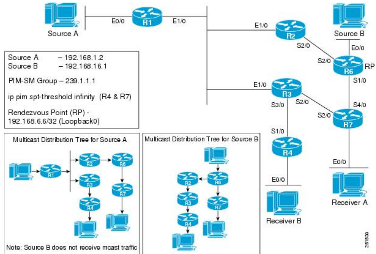
Figure 29: PIM-SM Example Topology: Active Sources and Interested Receivers (SPT Threshold Set to Infinity)
