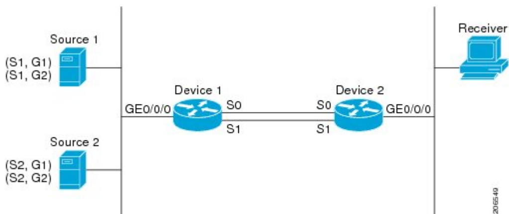
Figure 62: Default Behavior for IP Multicast When Multiple Equal-Cost Paths Exist
