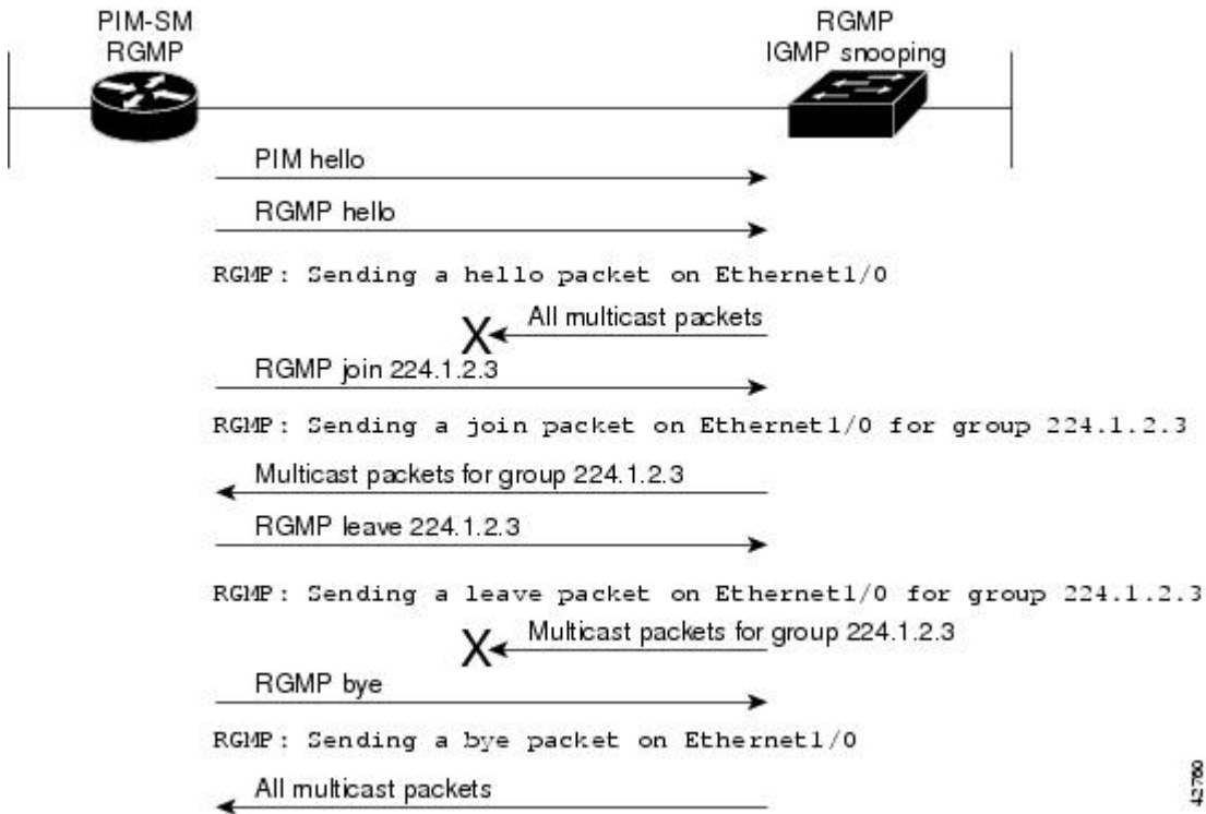
Figure 57: RGMP Debug Messages
