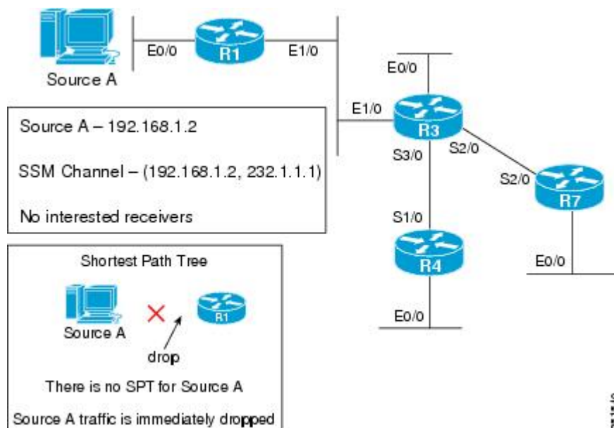
Figure 33: PIM-SSM Example Topology: Source Traffic Only with No Active Receivers
