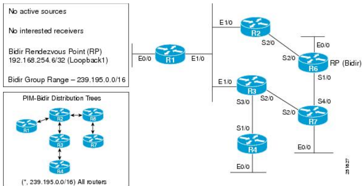
Figure 40: Bidir-PIM Example Topology: No Active Sources with No Interested Receivers
