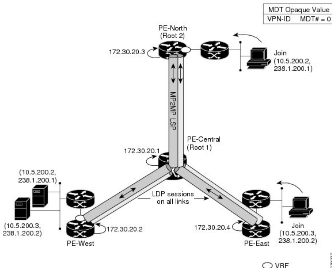
Figure 43: Default MDT Scenario
