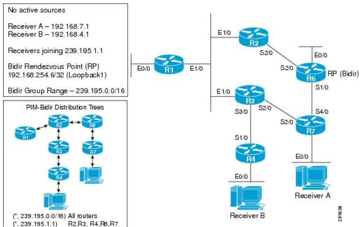
Figure 39: Bidir-PIM Example Topology: No Active Sources with Interested Receivers
