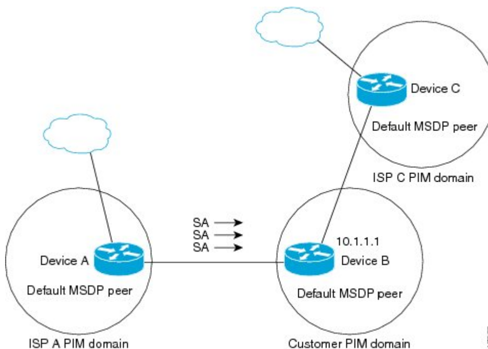
Figure 11: Default MSDP Peer Scenario
