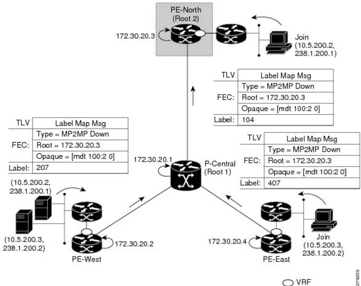
Figure 45: Default MDT Downstream--Root 2
