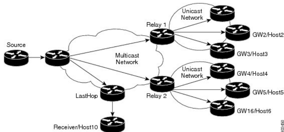
Figure 14: Automatic Multicast Tunneling (AMT)
