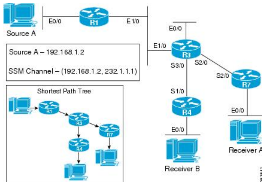
Figure 32: PIM-SSM Example Topology: Interested Receivers With or Without Active Sources
