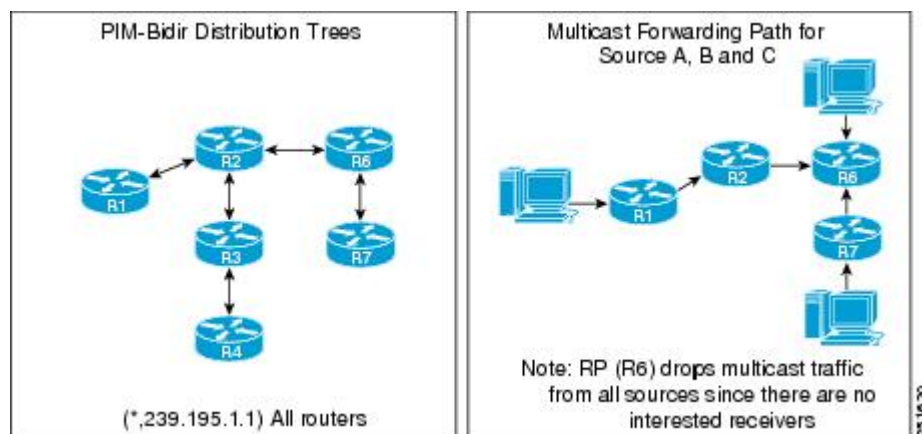
Figure 38: Bidir-PIM Distribution Trees and Multicast Forwarding Path for Active Sources with No Interested Receivers Example
