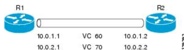
Figure 12: Two Routers with Back-to-Back PVCs
