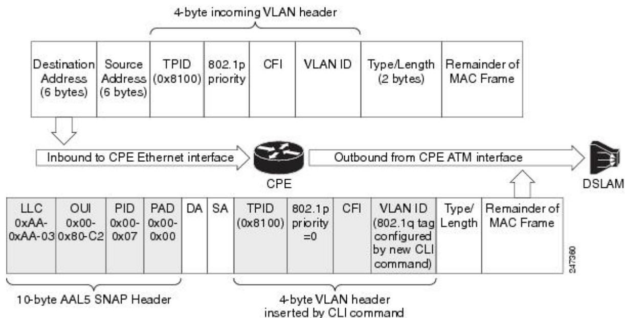
Figure 8: Incoming and Outgoing Packet Structures When an Incoming VLAN ID Is Present
