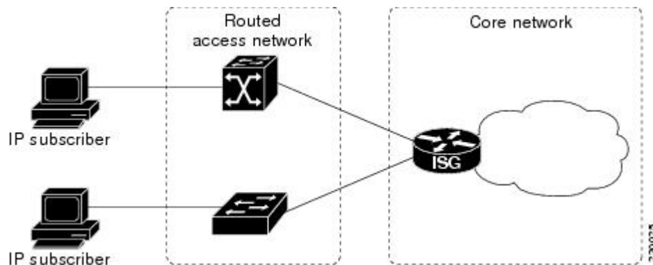
Figure 57: Routed Access Network
