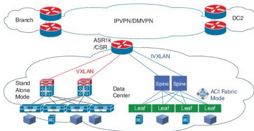
Figure 41: DCI EVPN Peer to ACI Spine
