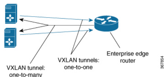
Figure 52: One-to-Many VxLAN Tunnels, Egress and Ingress
